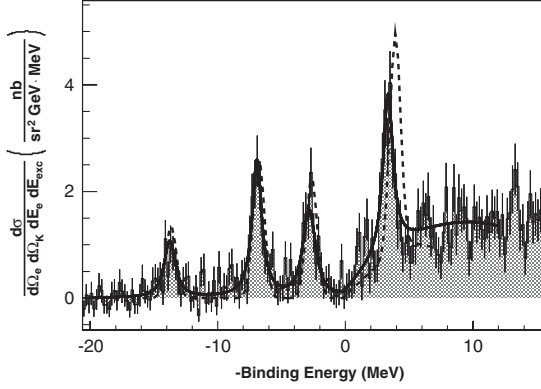
FIG. 3. The {}^{16}_{\Lambda}\text{N} binding-energy spectrum. The best fit using Voigt functions (solid curve) and a theoretical prediction (dashed curve) are superimposed on the data. See text for details.
