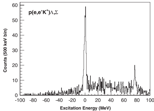
FIG. 1. Excitation energy spectrum of the p(e, e'K^+)\Lambda, \Sigma^0 on hydrogen, used for energy scale calibration. The fitted positions (not shown on the plot) for the peaks are -0.04 \pm 0.08 \text{ MeV} and 76.33 \pm 0.24 \text{ MeV} .
