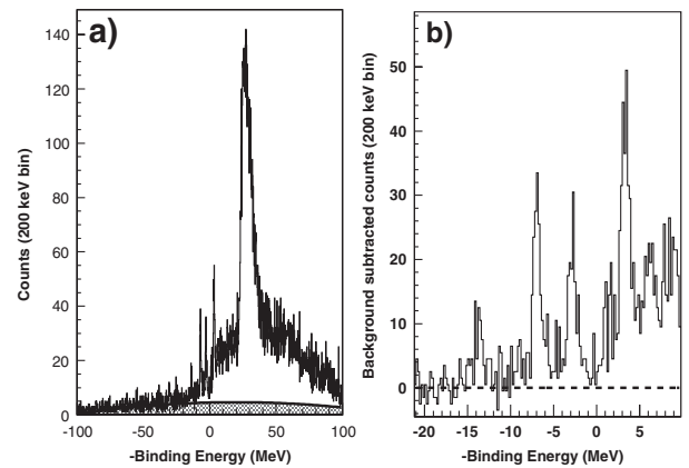
FIG. 2. The {}_{\Lambda}^{16}\text{N} binding-energy spectrum obtained after kaon selection with aerogel detectors and RICH. The electron-kaon random-coincidence contribution evaluated in a large timing window is superimposed on the spectrum in the left panel. The right panel shows the spectrum after this background has been subtracted.
