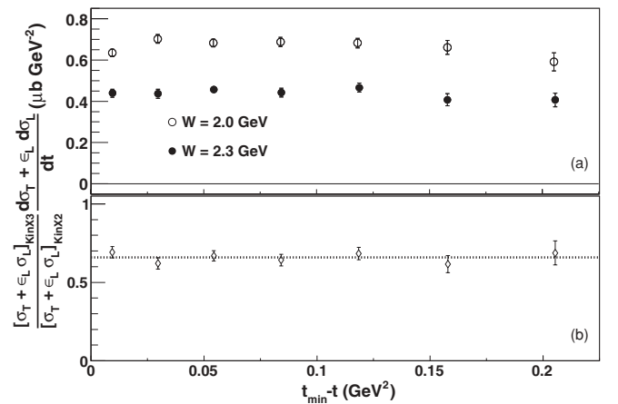
FIG. 12. (a) Separated H(e, e'\pi^0)p cross section \sigma_T + \epsilon_L \sigma_L as a function of t_{\min} - t for Q^2 = 2.1 \text{ GeV}^2 . Error bars represent statistical errors only. (b) Ratio of \sigma_T + \epsilon_L \sigma_L for the two kinematics as a function of t_{\min} - t . The fit of this ratio (dashed line) indicates the W dependence of the cross section.
