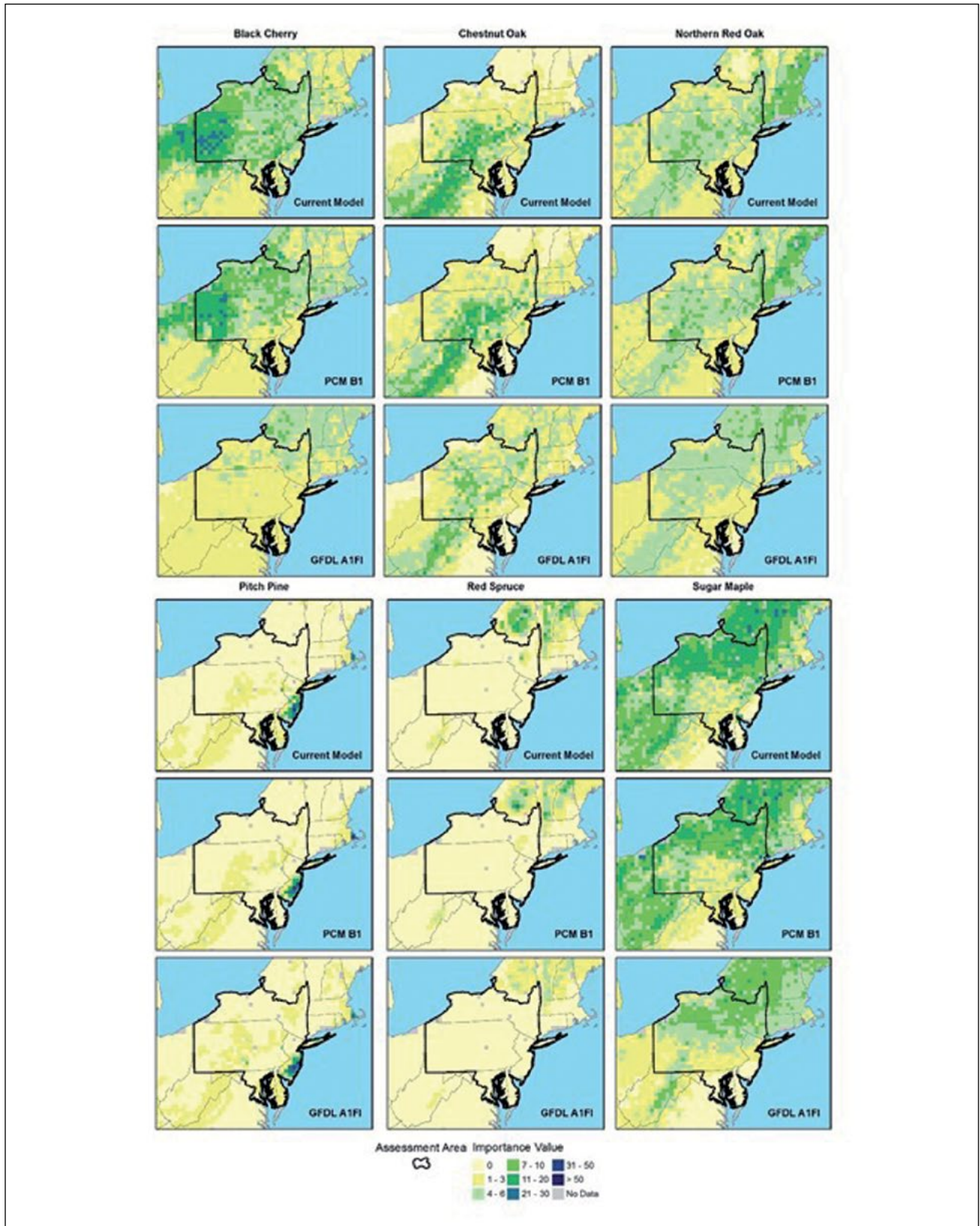
Figure 32.—Modeled importance values for six tree species. Maps show current importance values modeled by DISTRIB, using USDA Forest Service Forest Inventory and Analysis data (top) and projected for the end of the century (2070 through 2099) under PCM B1 (middle) and GFDL A1FI (bottom) climate model-emissions scenarios. Importance values can range from 0 to 100, with 0 indicating that the species is not present.
