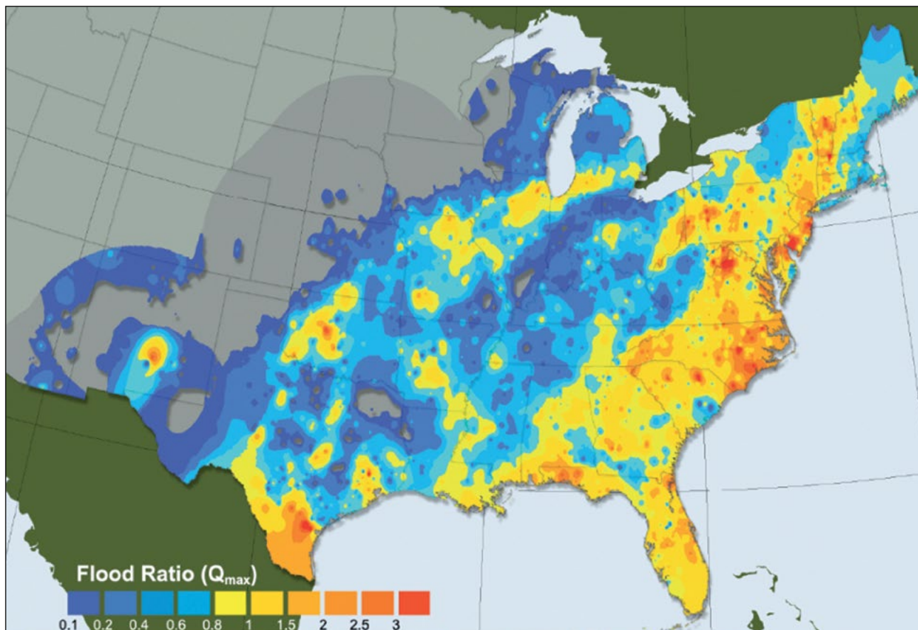
Figure 24.—Composite map of floods associated with hurricanes that made landfall from 1981 through 2011, based on stream gauge data. The flood ratio ( Q ) indicates the magnitude of departure from the 10-year flood peak; values larger (smaller) than 1 indicate floods were larger (smaller) than the 10-year flood peak. Figure adapted from data compiled by Villarini et al. (2014) and presented here from U.S. Global Change Research Program (2016).
