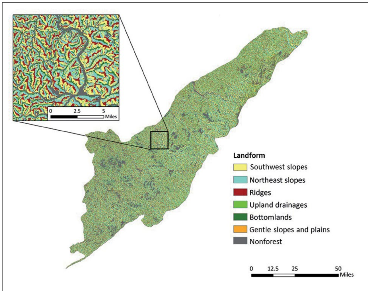
Figure 15.—Example landform map used in landscape initialization in the LANDIS PRO model (Dijak et al. 2016).
