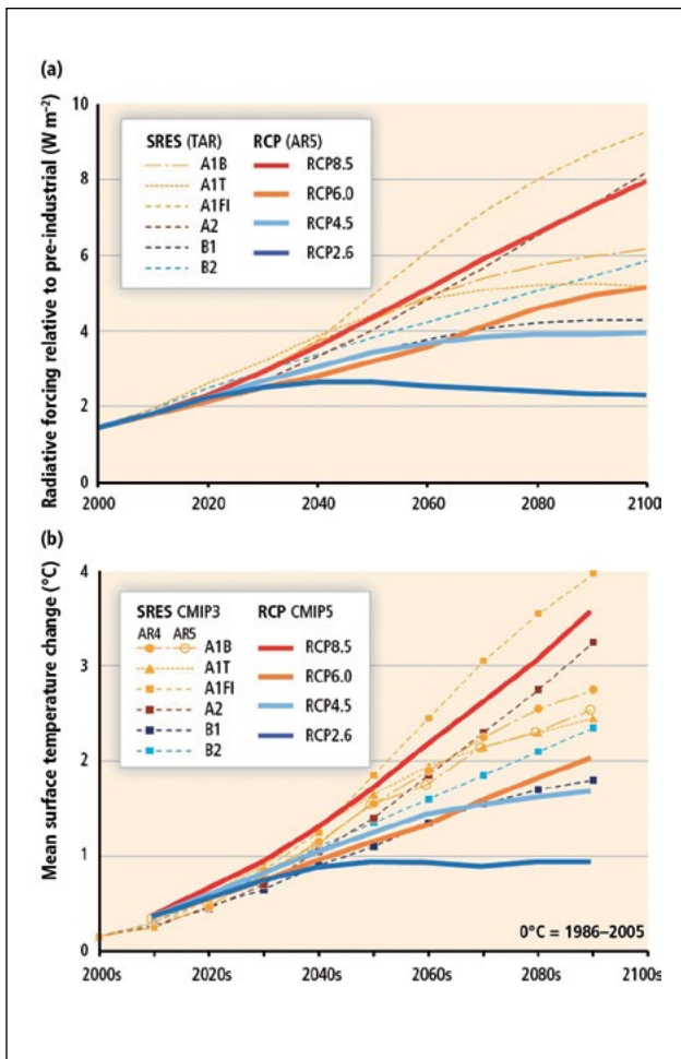
Figure 13.—(a) Projected radiative forcing (RF, W m^{-2} ) and (b) global mean surface temperature change ( ^{\circ}C ) over the 21st century using the Special Report on Emissions Scenarios (SRES) and Representative Concentration Pathway (RCP) scenarios. RF for the RCPs are taken from their published CO_2 -equivalent (Meinshausen et al., 2011), and RF for SRES are from the Third Assessment Report Appendix II (Table II.3.11). For RF derived from the Coupled Model Intercomparison Project Phase 5 (CMIP5) models, see WGI (Section 12.3; Tables AII.6.9, 6.10). The ensemble total effective RF at 2100 for CMIP5 concentration-driven projections are 2.2, 3.8, 4.8, and 7.6 W m^{-2} for RCP2.6, RCP4.5, RCP6.0, and RCP8.5, respectively. The SRES RF are shifted upward by 0.12 W m^{-2} to match the RCPs at year 2000 because the climate change over the 21st century is driven primarily by the changes in RF and the offset is due primarily to improvements in model physics including the aerosol RF. For more details and comparison with pre-SRES scenarios, see WGI AR5 Chapter 1 (Figure 1-15). Temperature changes are decadal averages (e.g., 2020s = 2016–2025) based on the model ensemble mean CMIP5 data for the RCPs (colored lines). The same analysis is applied to CMIP3 SRES A1B (yellow circles). See WGI AR5 Chapters 11, 12; Table AII.7.5. The colored squares show the temperature change for all six SRES scenarios based on a simple climate model tuned to the CMIP3 models (WGI AR4 Figure 10.26). The difference between the yellow circles and yellow squares reflects differences between the simple model and analysis of the CMIP3 model ensemble in parallel with the CMIP5 data. Figure courtesy of Burkett et al. (2014: 179); caption reused intact as requested (Burkett et al. 2014).
