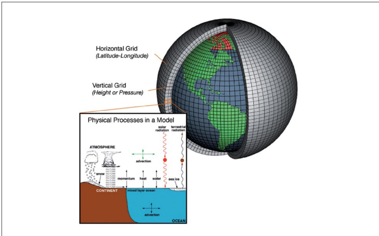
Figure 12.—Schematic describing climate models, which are systems of differential equations based on the fundamental laws of physics, fluid motion, and chemistry (NOAA 2017b). The planet is divided into a three-dimensional grid that is used to apply basic equations; atmospheric models calculate winds, heat transfer, radiation, relative humidity, and surface hydrology within each grid and evaluate interactions with neighboring points.
