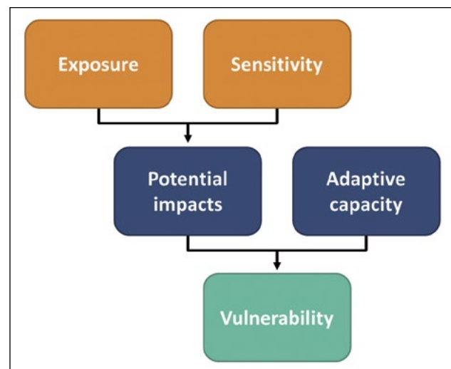
Figure 36.—Key components of vulnerability, illustrating the relationship among exposure, sensitivity, and adaptive capacity. Adapted from Glick et al. (2011).
