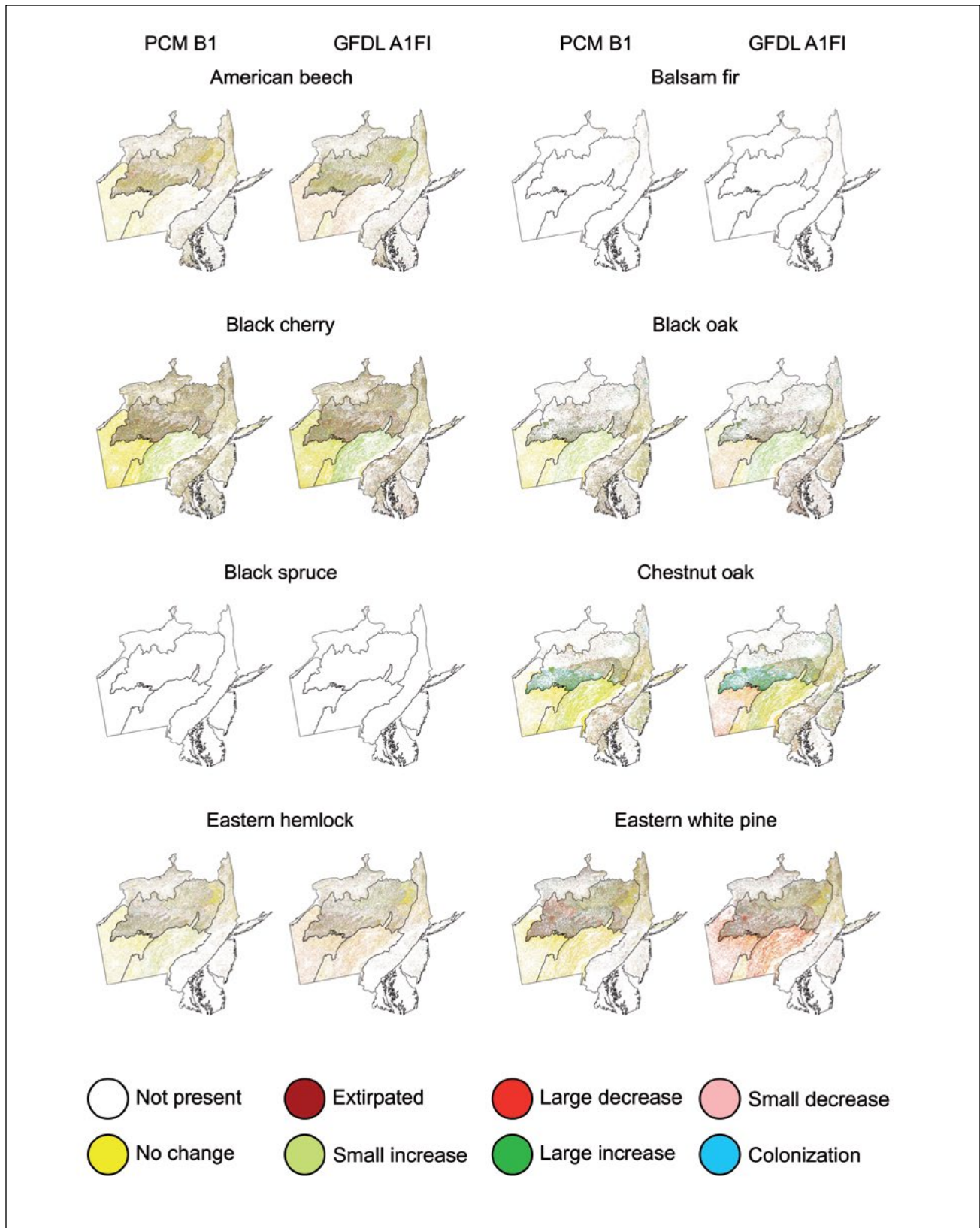
Figure 58.—Change in basal area projected by the LANDIS PRO model for 22 species under two climate model-emissions scenario combinations at year 2100 relative to a current climate scenario (1980 through 2009). Assessment area values were derived from the weighted average of sections.
