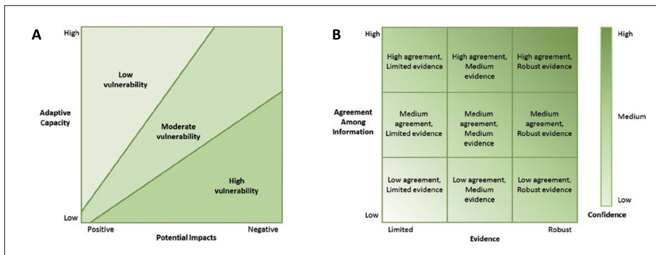
Figure 60.—Figure used for (A) vulnerability determination by expert panels, based on Swanston and Janowiak (2016) and described by Brandt et al. (2017); and (B) confidence rating among expert panels, adapted from Mastrandrea et al. (2010).
