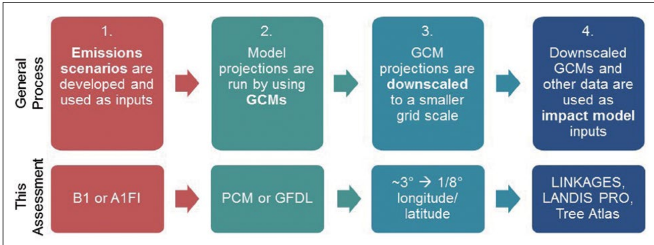
Figure 14.—Steps in the development of forest impact models using projections from general circulation models (GCMs) and specific steps taken in this assessment.
