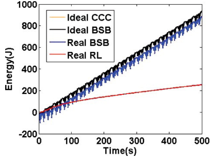
Figure 5.6: The extracted energy using SA control and EKF
