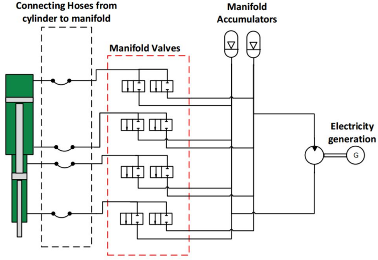
Figure 6.1: The layout of the Discrete Displacement Cylinder (DDC) hydraulic system.
