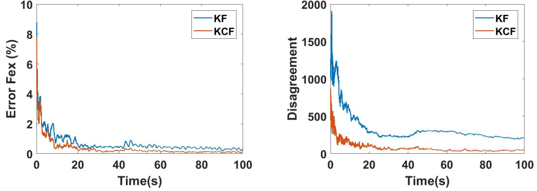
Figure 5.16: The average percent estimation error and the disagreement of the excitation force using 200 frequencies
