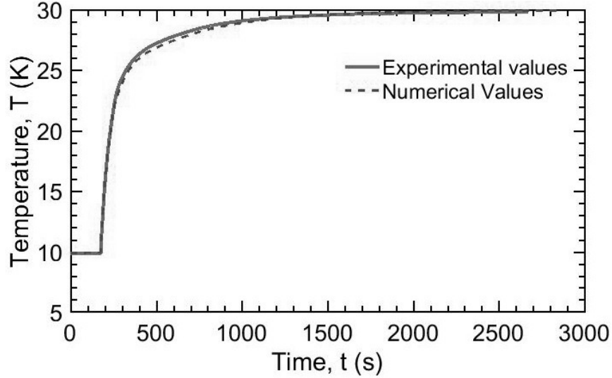
Figure 2.4: Experimental and numerical time response for the dry cell experiment with the 10 mm diameter 316L SS test cell.
