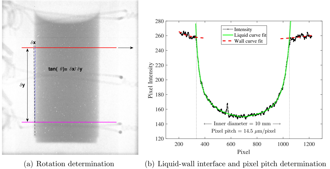
Figure 3.4: Determination of (a) rotation & (b) liquid-wall interface and pixel pitch using pixel intensities shown by the red line and arrow. The image represents liquid hydrogen at 21K in a 10 mm Al6061 test cell.
