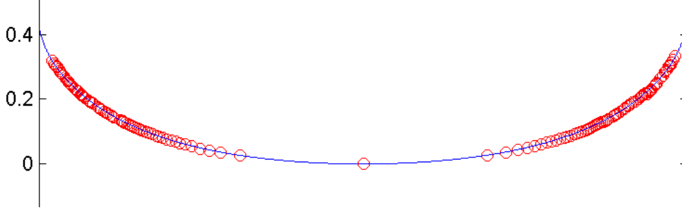
Figure 2.6: Laplacian curve fit to the detected meniscus edge on stacked image of liquid hydrogen in Aluminum test cell. Symbols are the meniscus edge and the line is the Laplace curve representing the best fit to the edge data.
