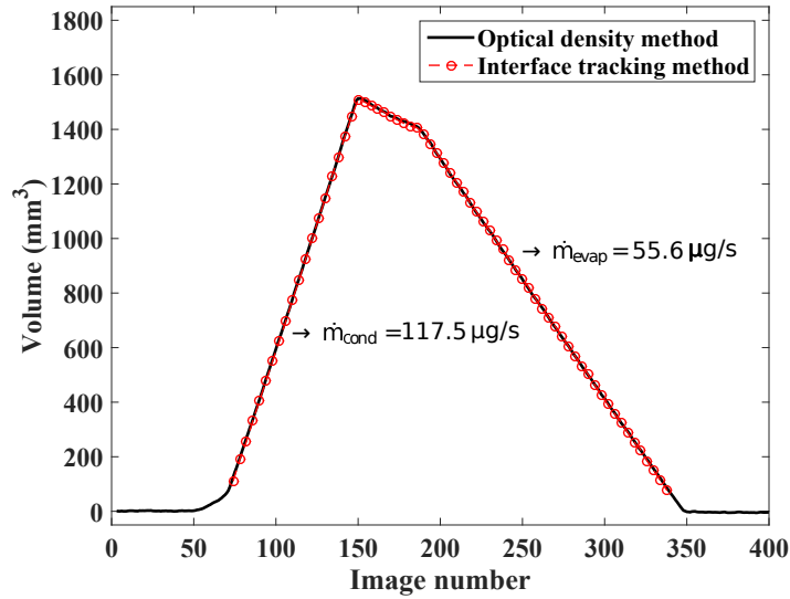
Figure 3.12: Phase change rates for hydrogen in the 10 mm Al cell saturated at 21 K. Condensation test is conducted at 19 K and evaporation at 23 K
