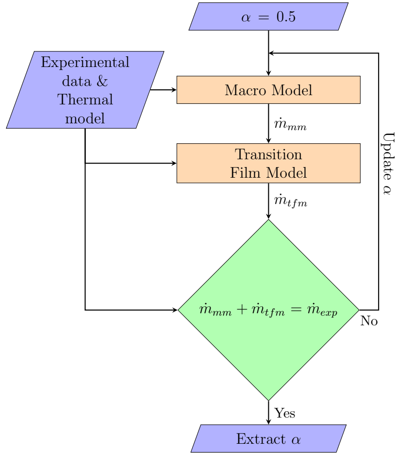
Figure 5.8: Algorithm flowchart
