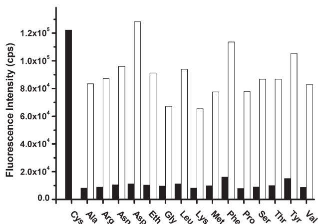
Fig. 6 Fluorescence response of BODIPY dye G b (10 \mu M) to various amino acids (5 mM) at 677 nm. Conditions: 0.01M PBS buffer pH 7.4 solution. \lambda_{\text{ex}} = 620 nm. Black bars represent the addition of various amino acids to G b solution. White bars represent the further addition of cysteine (5 mM) to the above solutions, respectively.
