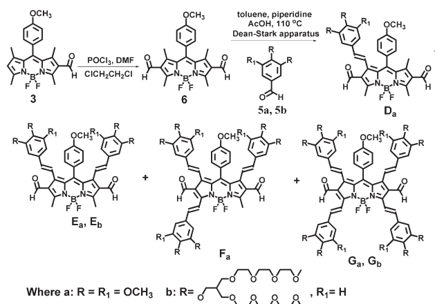
Scheme 2 Synthetic route to 2,6-diformyl-BODIPY dyes bearing different numbers of styryl groups.
