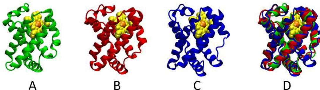
Figure 2. Structures of proteins from the globin family of proteins as an example of divergent evolution . A. Human hemoglobin, in red blood cells of human circulatory system (1HBB), B. Sperm whale myoglobin, in muscle (1MBD), C. Lupine leghemoglobin, in legumes (1GDJ), and D. Overlay of all three structures. The structural similarities of all three proteins are evident upon comparison of individual structure or by overlaying all three structures. There is a very large percent of similarity protein structure. This is an indication of divergent evolution in which these globin proteins evolved from a common ancestor composed of the same structural fold. Figures were rendered using VMD.
