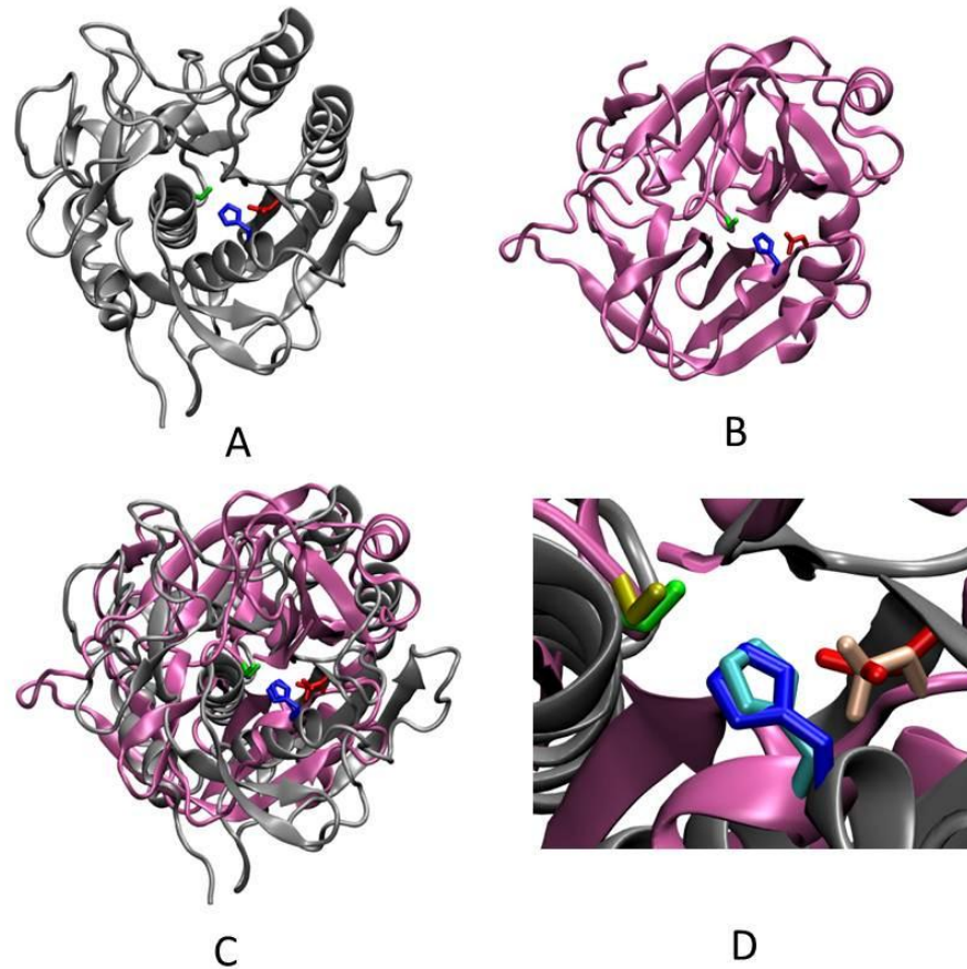
Figure 3. Structures of serine protease proteins as an example of convergent evolution . A. Chymotrypsin (1GCT), B. Subtilisin (1SUP), C. Overlay of chymotrypsin and subtilisin, and D. Zoomed in view of chymotrypsin-subtilisin overlay focusing on the catalytic triad of both enzymes. The overall structures of these two proteins are very different, as it is evident by the side-by-side comparisons of the structures (A and B) and the overlay of them (C), indicating that chymotrypsin and subtilisin do not have similar evolutionary origins. The catalytic triad, however, composed of three strategically placed amino acids (highlighted in D) is very similar between the two proteins, enabling these two very different proteins to catalyze the same type of reaction. This is indicative of an advantageous structural arrangement that was evolutionary adapted into two unrelated proteins.
