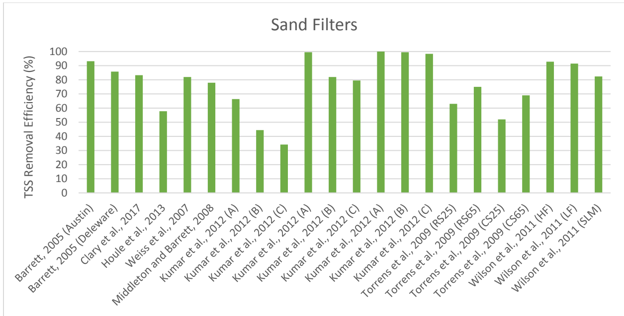
Figure 10 - TSS Percent Removal Efficiency for Sand Filters, as derived from previous studies
