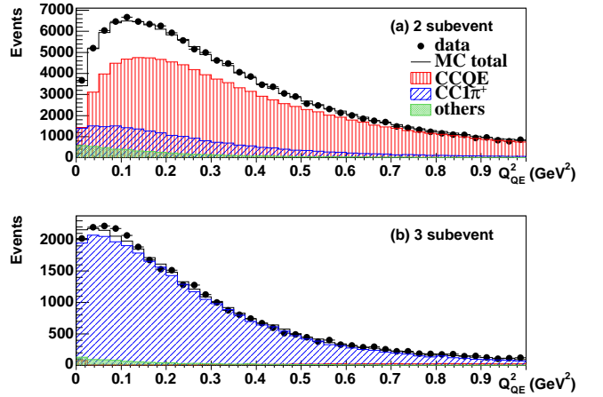
FIG. 8: (color online) Distribution of events in Q^2_{QE} for the (a) 2 and (b) 3 subevent samples after the application of the data-based CC1\pi^+ background constraint and the new CCQE model parameters M_A^{\text{eff}} and \kappa as determined from the CCQE fit procedure described in the text.
