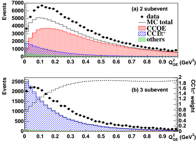
FIG. 7: (color online) Distribution of events in Q^2_{QE} for the (a) 2 and (b) 3 subevent samples before the application of the CC1\pi^+ background correction. Data and MC samples are shown along with the individual MC contributions from CCQE, CC1\pi^+ , and other channels. In (b), the dashed line shows the CC1\pi^+ reweighting function (with the y-axis scale on the right) as determined from the background fit procedure.
