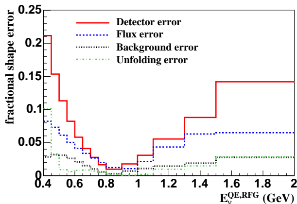
FIG. 16: Fractional shape error on the MiniBooNE \nu_\mu CCQE flux-unfolded cross section separated into major components. The overall normalization error of 10.7% is not shown.
