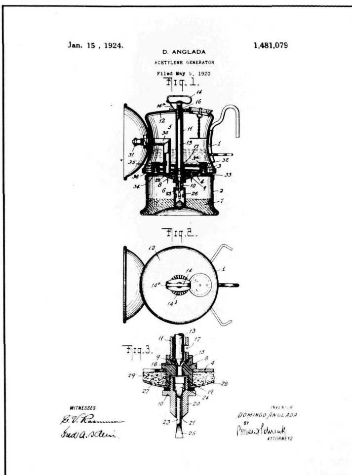
Wolf cap lamp patent
