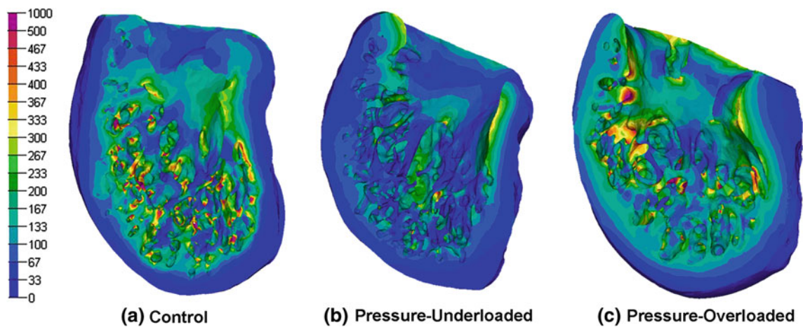
Fig. 4 Color contour plots of calculated von Mises stress for a characteristic model in each of the three groups. Bar scale shows stress in Pa. Scaling is not necessarily equivalent on all models, and cutting planes were chosen to show maximal interior view
