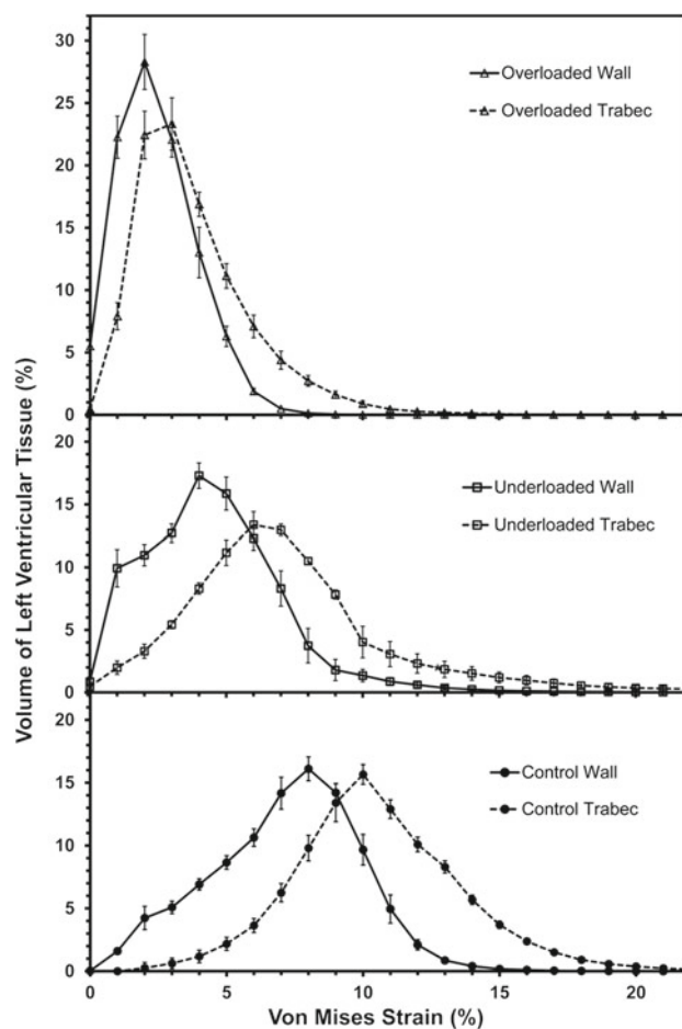
Fig. 10 Histograms of percentage of left ventricular tissue volume versus von Mises strain for both ventricular wall and trabecular tissue for the three treatment groups. Values are mean \pm SE of all models in the group
