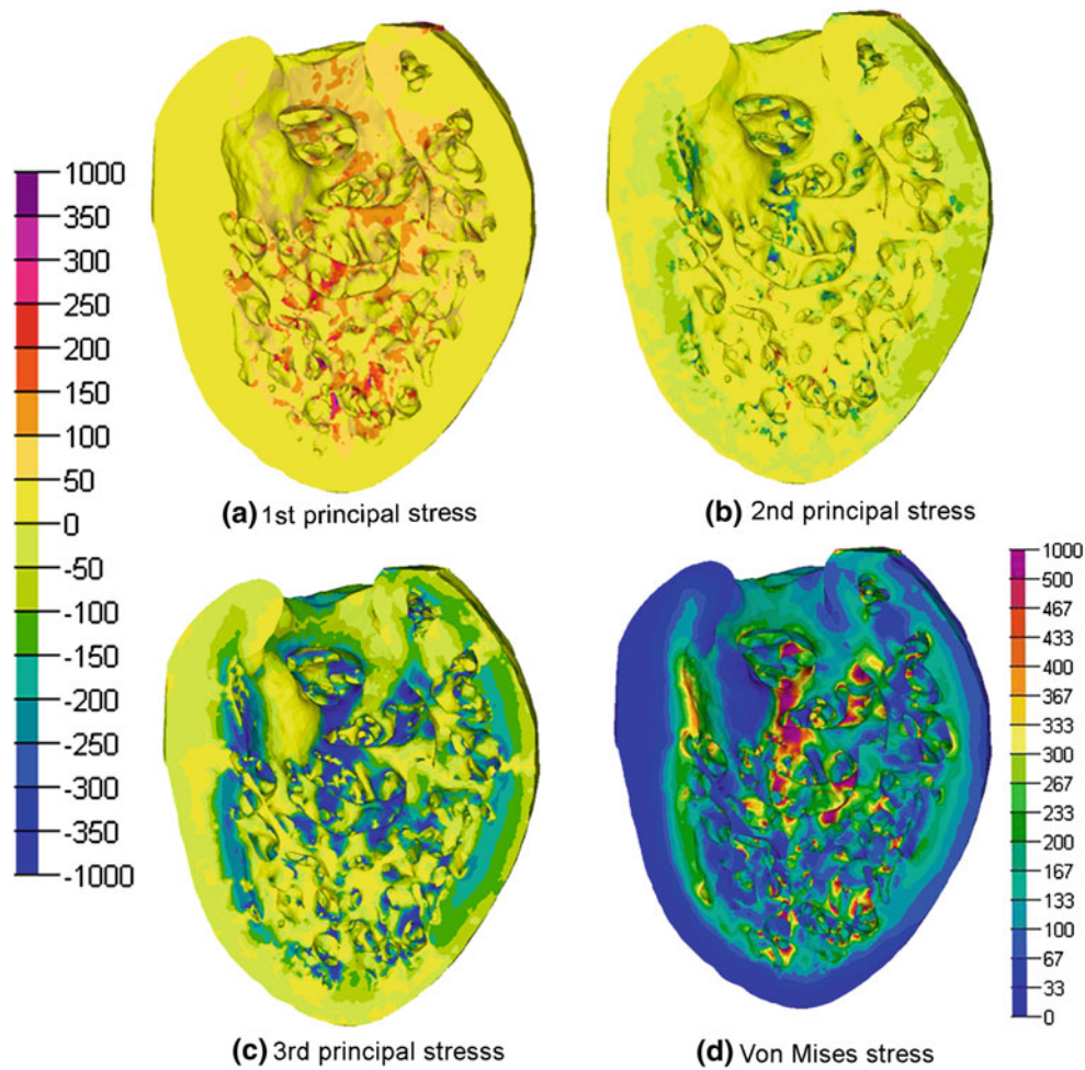
Fig. 7 Color contour plots of four different stress measures for a single heart in the control group. Bar scale at left denotes stress in Pa for cases a, b, and c. Bar scale in lower right denotes stress in Pa for case d
