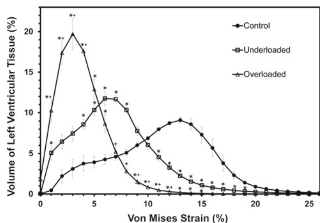
Fig. 9 Histogram of percentage of left ventricular tissue volume versus von Mises strain. For clarity, results are shown as bin height plotted versus the bin center and points are connected. Values are mean \pm SE of all models in the group. * denote percentage volume of the overloaded or underloaded models is significantly different from the control group at the specific strain bin ( p < 0.05 ). + denotes percentage volume of overloaded models is significantly different from that of underloaded models at the specified strain bin ( p < 0.05 )
