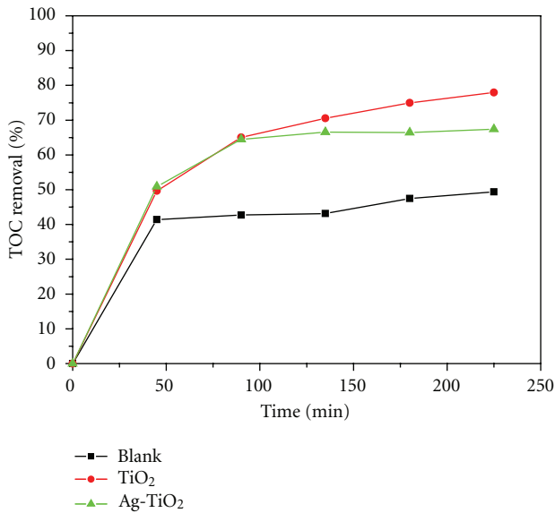
FIGURE 10: TOC removal percentage of E. coli versus UV light irradiation by using TiO 2 and Ag-TiO 2 as photocatalysts.
