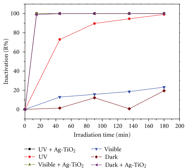
FIGURE 7: R percentage versus irradiation time of different light sources using \text{Ag-TiO}_2 as photocatalysts.
