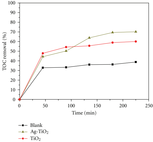
FIGURE 9: TOC removal percentage of E. coli versus visible light irradiation by using TiO 2 and Ag-TiO 2 as photocatalysts.
