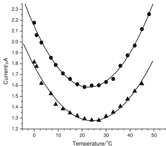
Fig. 5 Current response as a function of temperature for PC only (filled circle) and for the 60/40 mol% PC/cholesterol film (filled triangle); solid curves are second order polynomials fitting curves modeling the two regime behavior of the current response of the redox probe in the film
