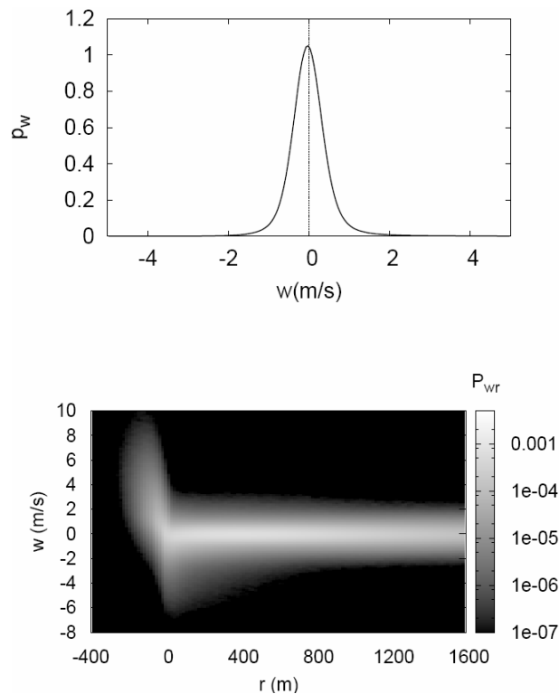
Fig. 13. Vertical velocity distribution in the cumulus cloud layer (top) and vertical velocity distribution as a function of distance to cloud (bottom).
