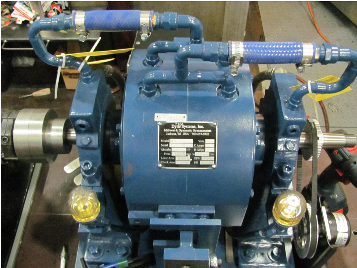
Figure 10 Midwest Model 46 dynamometer
