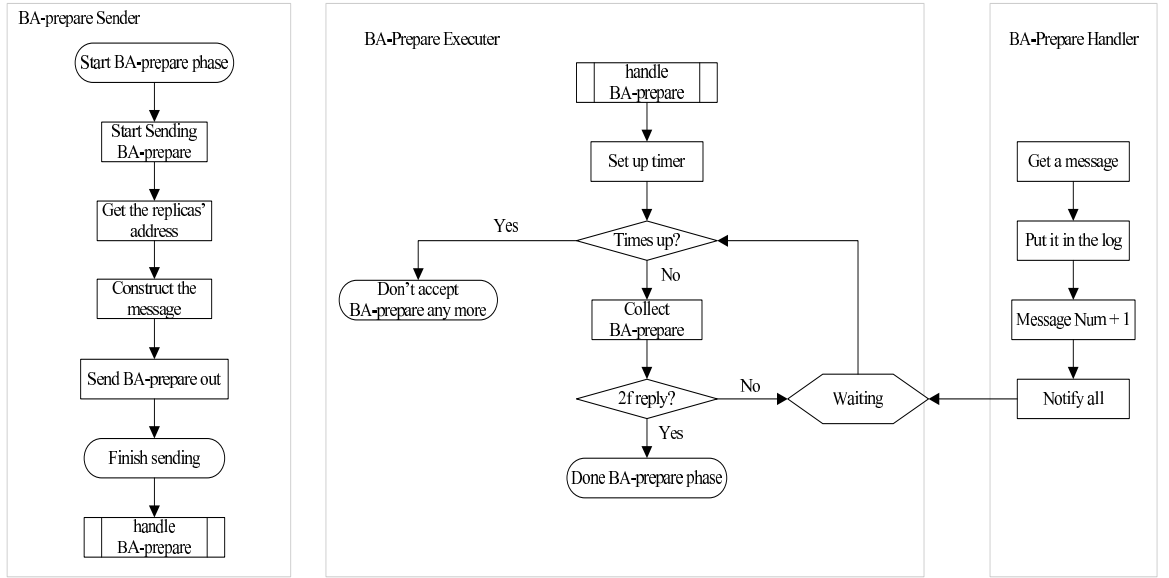
Figure 15: Flowchart of BA-prepare phase for Activation Service
