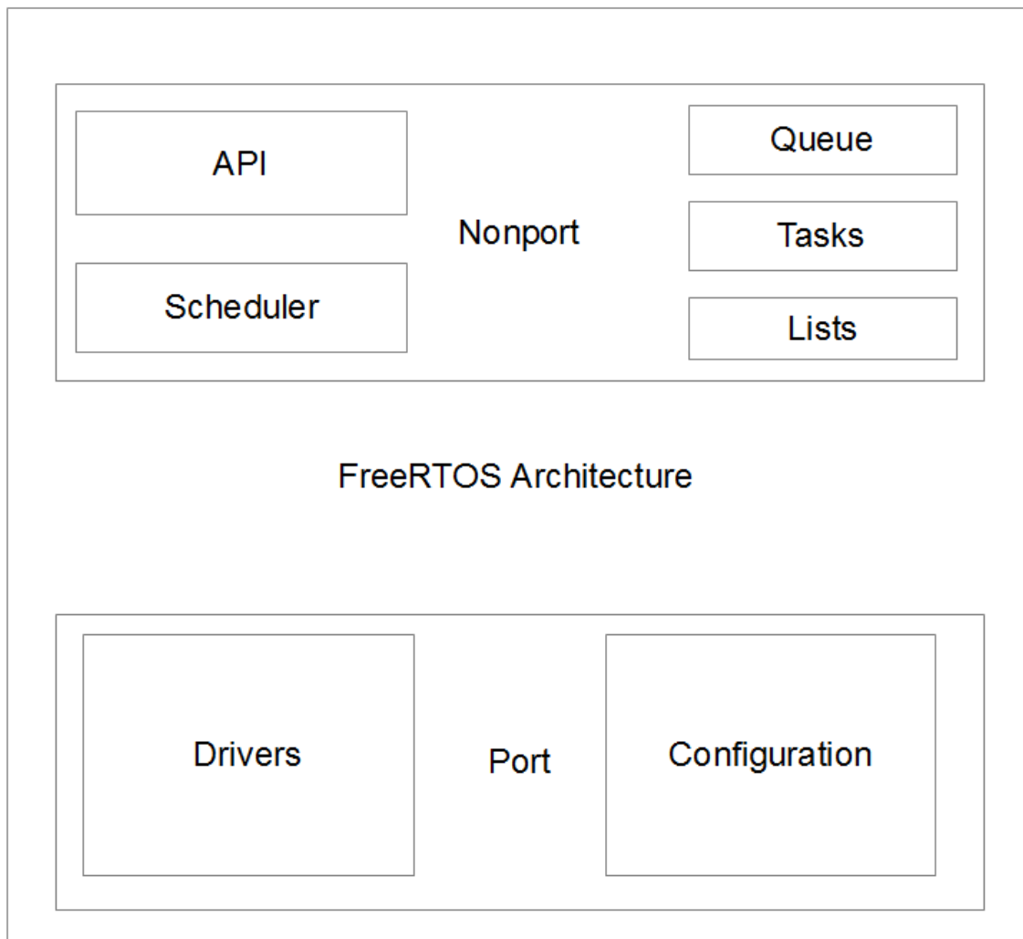
Figure 1: FreeRTOS Architecture
