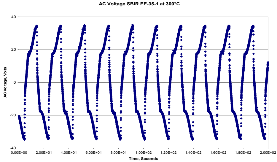
Figure 69. EE-35- 1 Alternator Voltage at 300° C
