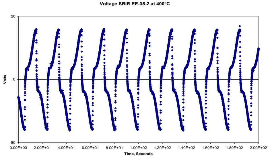
Figure 67. EE-35- 2 Alternator Voltage at 400° C
