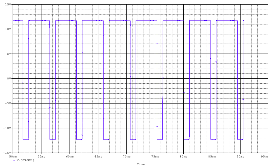
Figure 46. Buck Converter with Zener MOSFET Switching Stage One
