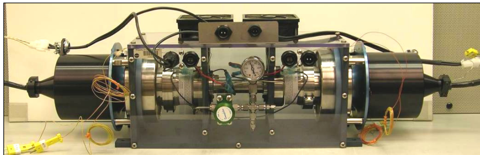
Figure 5. ASRG Simulator Setup [4]
