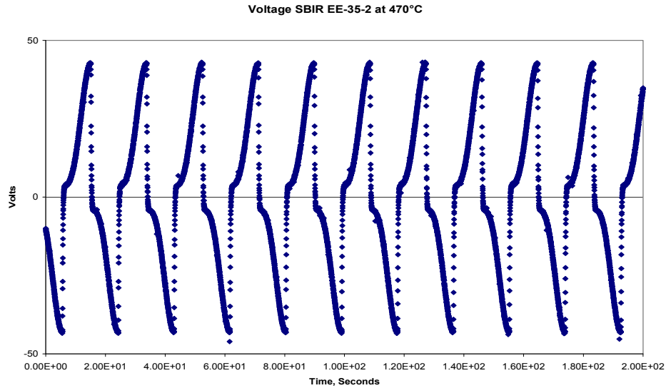
Figure 64. EE-35- 2 Alternator Voltage at 470° C
