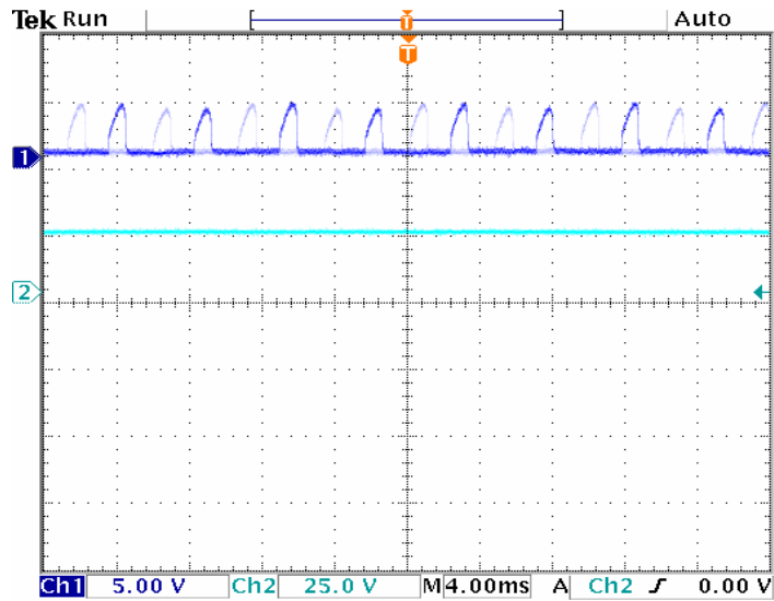
Figure 59. Op-Amp Stage and DC Output Voltage: Bench Testing
