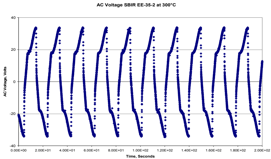
Figure 70. EE-35-2 Alternator Voltage at 300° C
