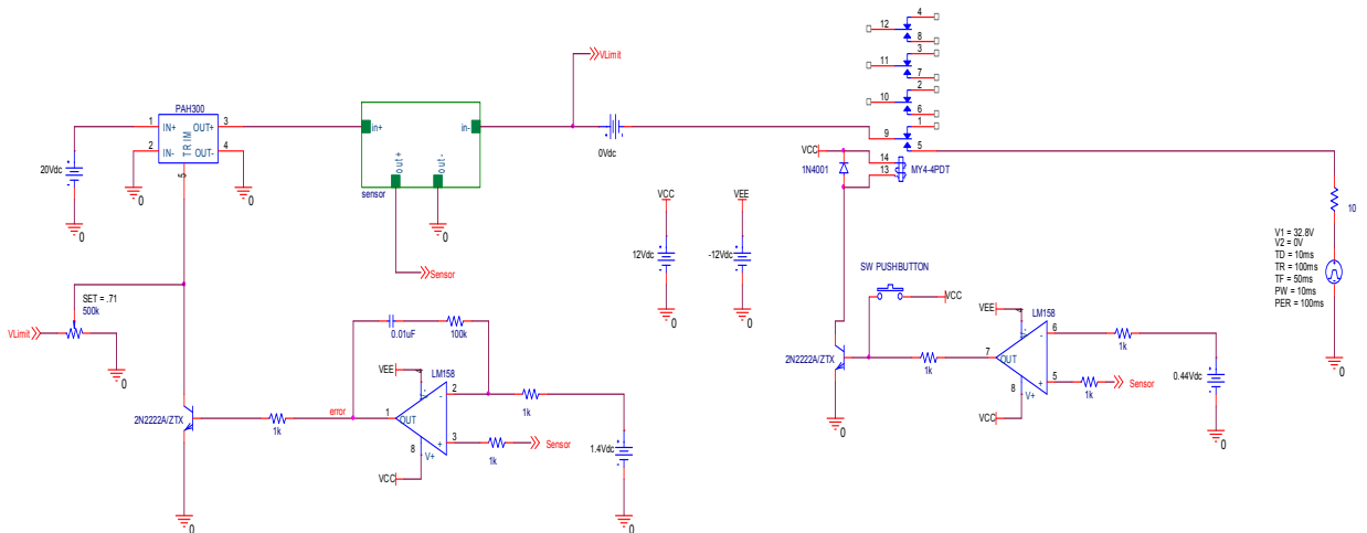
Figure 95. Battery Charger Final Design
