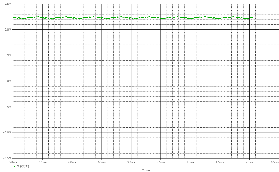
Figure 44. Buck Converter with Zener DC Output Voltage
