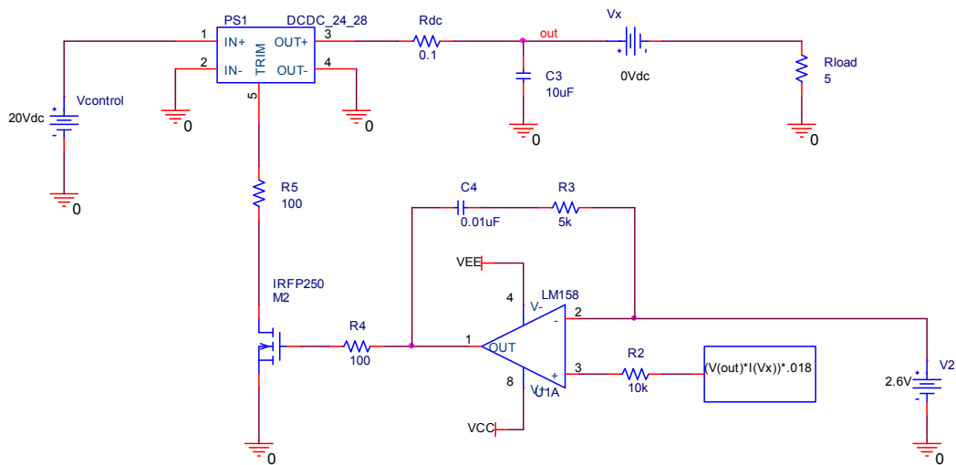
Figure 80. Fourth Step in Constant Power Circuit Design Process
