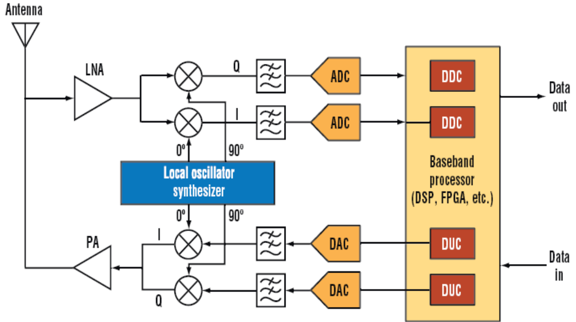
Figure 8: Functional representation of an SDR
