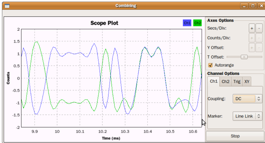
Figure 21: The combined symbol at the destination node
