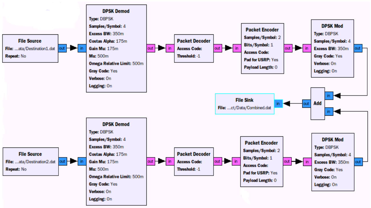
Figure 17: Combination of the received signal in two time slots (Combine.grc)
