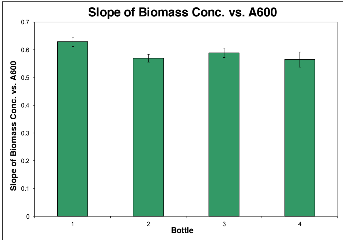
Figure 17: Slope of biomass concentration versus absorbance for each of the growth bottles. Average slope was 0.59 \pm 0.03 gdw/L*A 600 . The error bars are standard errors calculated using Excel's Linest function.
