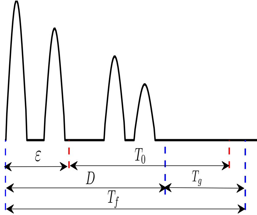
Figure 27: A GFSK frame structure in the presence of synchronization errors
