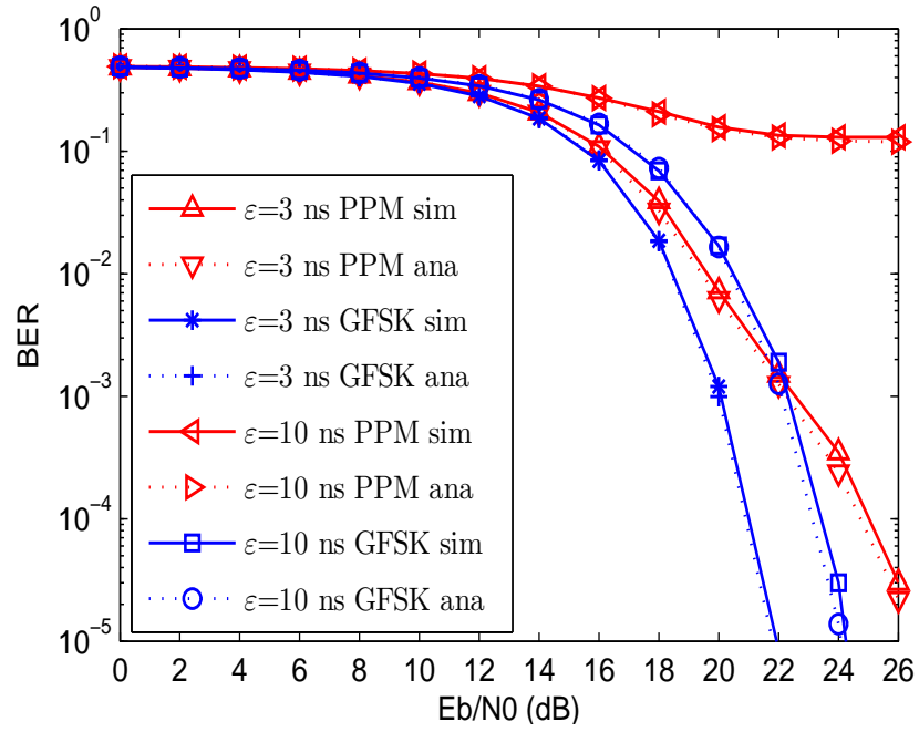
Figure 90: Comparison of BER performance of GFSK and PPM in multipath channels (CM4 model, D = 80 ns, \varepsilon = 3 and 10 ns)
