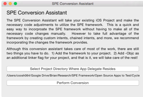
Fig. 6. Screenshot of SPE Conversion Assistant converting an open source application.
