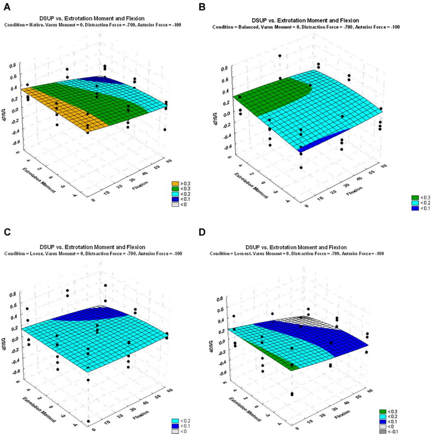
Figure 4. Effect of flexion and external rotation on superior motion for (A) native knee, (B) balanced TKA, (C) loose condition TKA, and (D) loosest condition TKA. Other variables held constant (varus moment = 0 Nm; compression = 700 N; posterior drawer = 100 N).
