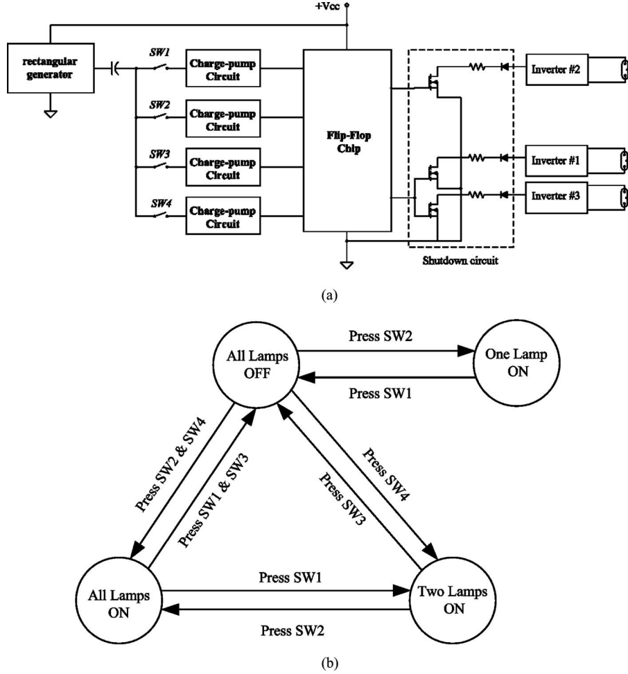
Fig. 3. (a) Block diagram of the dimming control circuit. (b) State machine of dimming control unit.
