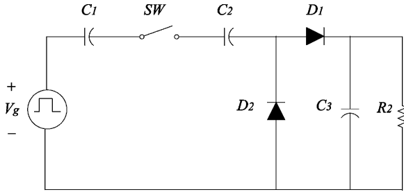
Fig. 5. Topology of the charge pump circuit.
