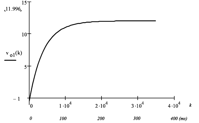
Fig. 10. Charge pump output voltage waveform (MathCAD result).
