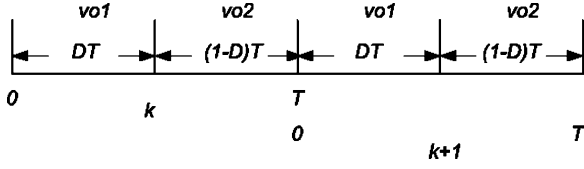
Fig. 9. Time sequence diagram of the charge pump output voltage.
