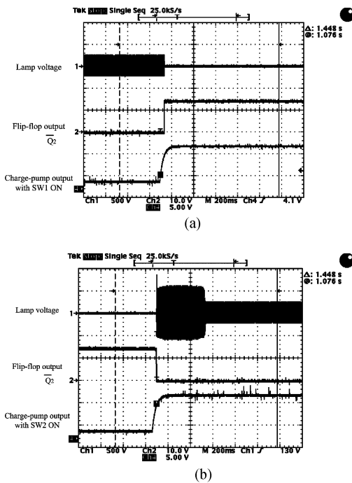
Fig. 14. (a) Lamp #2 voltage with OFF signal. (b) Lamp #2 voltage with ON signal.
