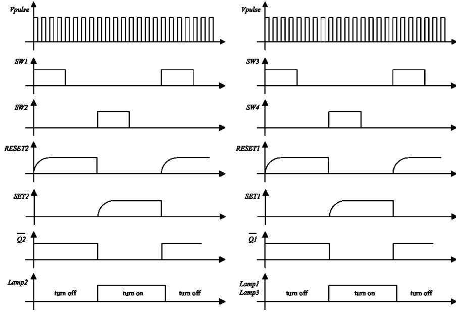
Fig. 4. Timing diagram of proposed digital dimming controller.
