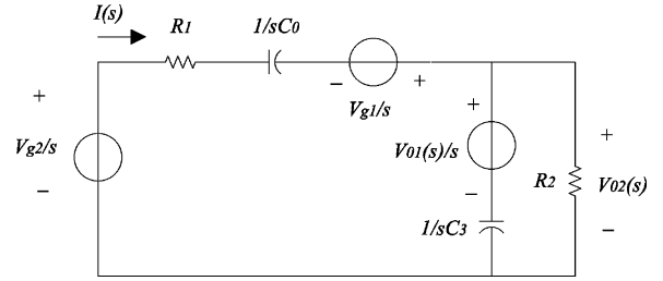
Fig. 8. Laplace transformed equivalent circuit in mode II.
