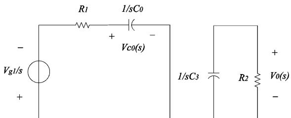
Fig. 7. Laplace transformed equivalent circuit in mode I.
