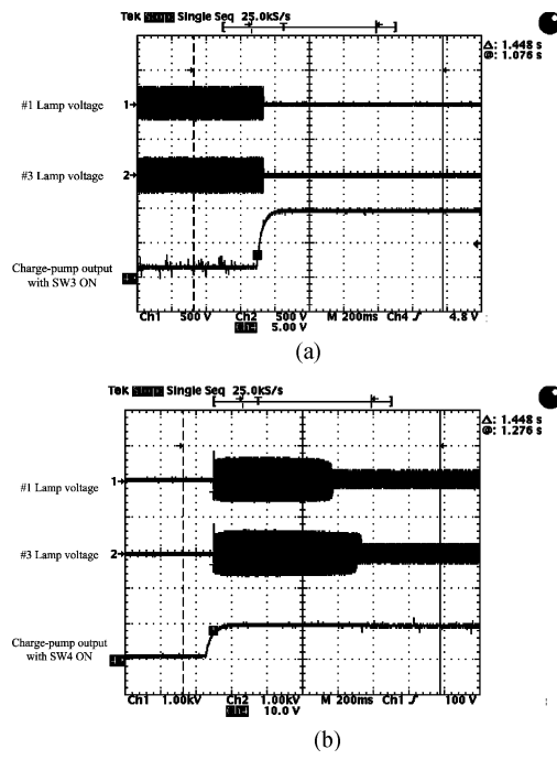
Fig. 15. (a) Lamp #1, #3 voltages with OFF signal. (b) Lamp #1, #3 voltages with ON signal.
