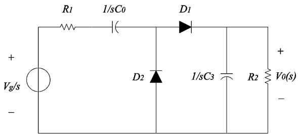
Fig. 6. Charge pump Laplace transformed equivalent circuit.
