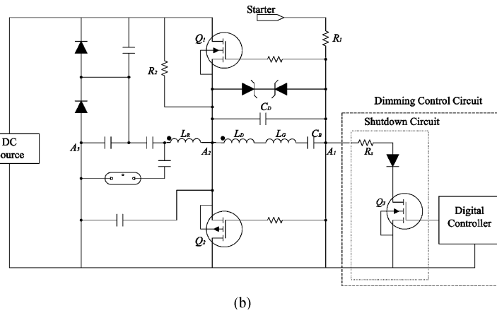
Fig. 13. (a) Proposed schematic of a digital dimming controller. (b) Schematic diagram of one inverter stage with a proposed dimming controller.
