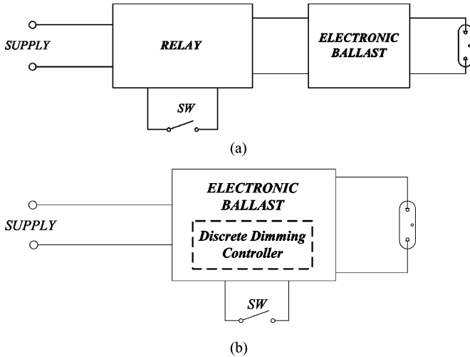
Fig. 1. (a) Conventional lighting system. (b) Proposed dimming system.
