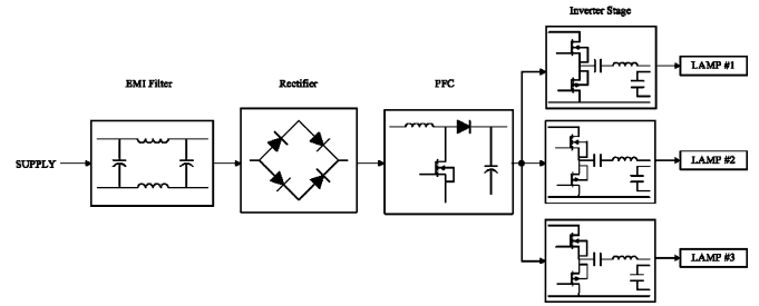
Fig. 2. Block diagram of the ballast module.
