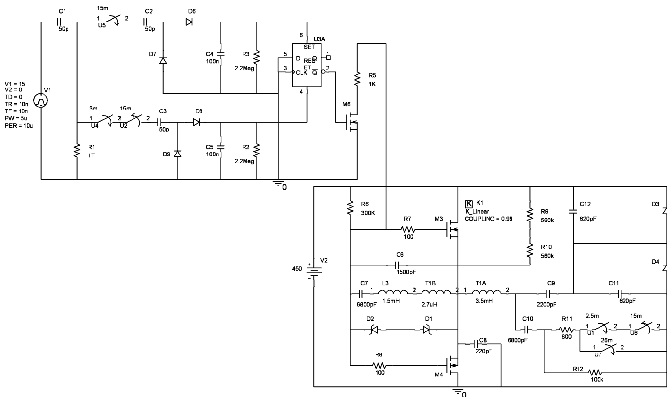
Fig. 11. PSPICE model of the proposed discrete dimming ballast.
