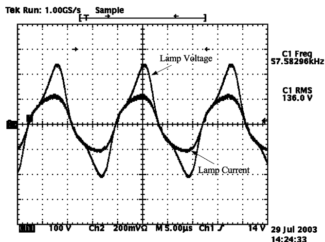
Fig. 16. Lamp voltage and current of the discrete dimming ballast (experimental results).
