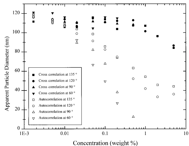
Fig. 9. Particle diameter inferred from autocorrelation and cross-correlation functions by use of a two-cumulant fit for measurements made at scattering angles of 60^\circ , 90^\circ , 120^\circ , and 135^\circ .
