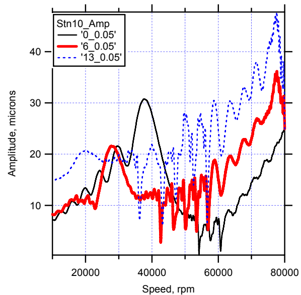
Figure 12: Deceleration data for 0.05 sec ramp time.
