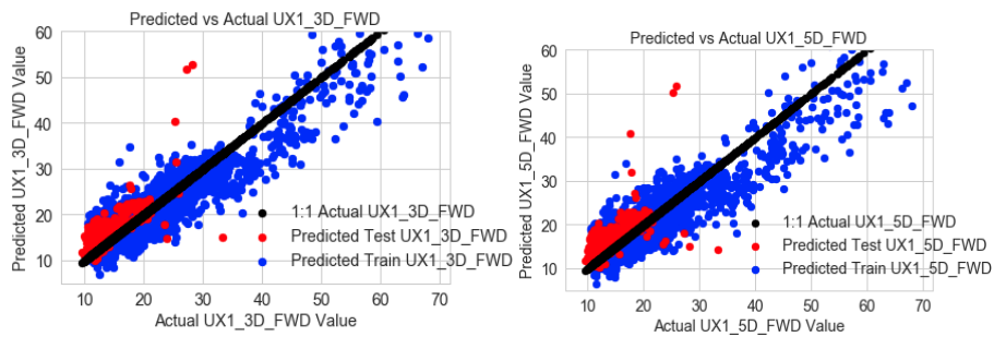
Fig. A14.1. SVR Scatter Plot of Training & Test Actual vs. Estimated for 1-mth VIX Futures (UX1) 3 and 5-days Forward (Jul 2006 to Jun 2015 for Train & Jun 2015 to Jun 2018 for Test)
