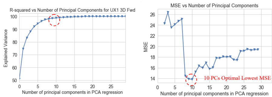
Fig. 15. PCA Reduction to 10 Principal Components (PCs) with Explained Variance over 90% for 1-mth VIX Futures (UX1) 3 and 5-days Fwd. In addition, the second graph shows that with 10 PCs the MSE is minimized for both 3 and 5-days Fwd. (Jul 2006 to Jun 2015)
