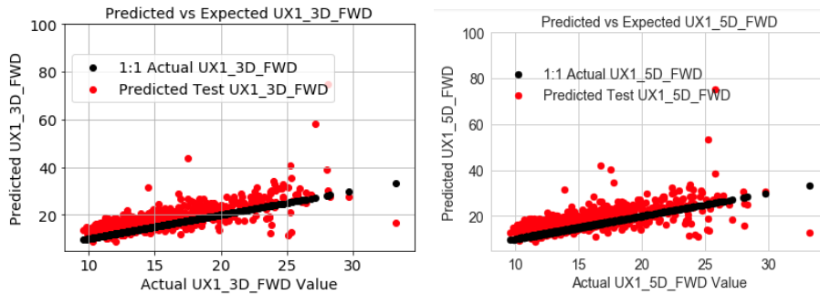
Fig. A9.2. MLR Scatter Plot of Test Actual vs. Estimated for 1-mth VIX Futures (UX1) 3 and 5-days Forward (Jun 2015 to Jun 2018)
