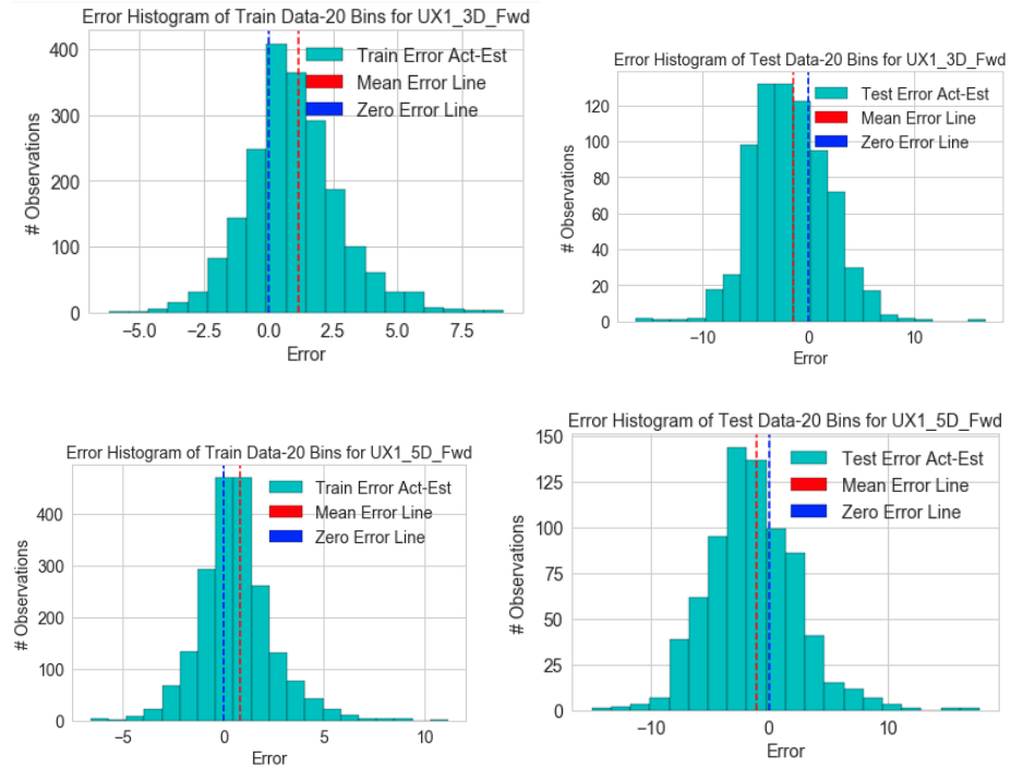
Fig. A15.4 RNN Error Histogram of Estimated Training vs. Actual Training and Test vs. Actual Test for 1-mth VIX Futures (UX1) 3 and 5-day Forward (Jul 2006 to Jun 2015 for Train & Jun 2015 to Jun 2018 for Test)
