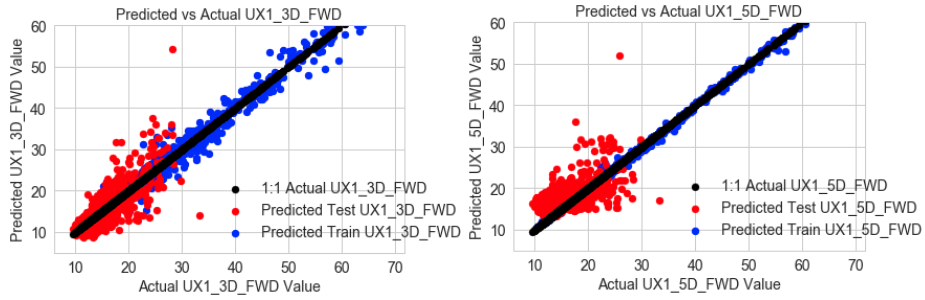
Fig. A12.2 Ensemble Scatter Plot of Training & Test Actual vs. Estimated for 1-mth VIX Futures 3 and 5 days Forward
