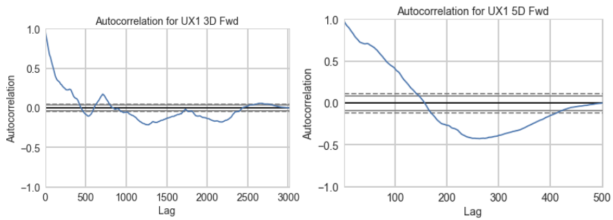
Fig. A11.3 ARIMA Optimal Autocorrelation Lag for 1-mth VIX Futures (UX1) 3 and 5-days Forward (Jun 2006 to Jun 2015 for Train)
