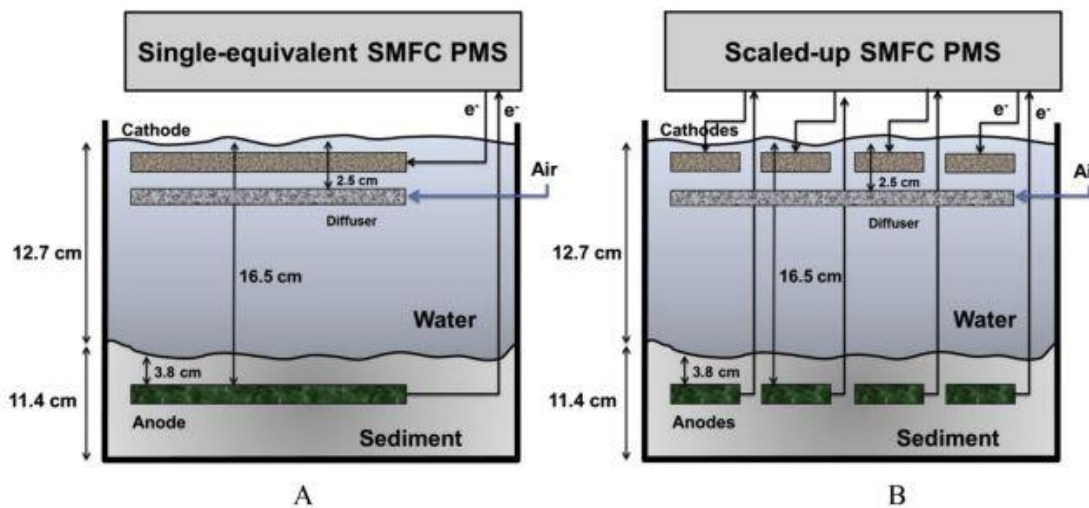
Figure 11. Schematic of (A) a single-equivalent SMFC and (B) a scaled-up SMFC. 2
