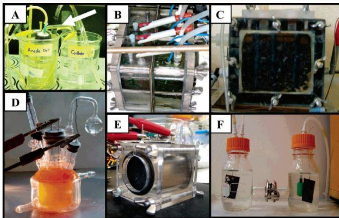
Figure 1. “Types of MFCs used in studies: (A) easily constructed system containing a salt bridge (shown by arrow); (B) four batch-type MFCs where the chambers are separated by the membrane (without a tube) and held together by bolts; (C) same as B but with a continuous flow-through anode (granular graphite matrix) and close anode-cathode placement; (D) photoheterotrophic type MFC; (E) single-chamber, air-cathode system in a simple “tube” arrangement; (F) two-chamber H-type system showing anode and cathode chambers equipped for gas sparging.” 1 [citations removed]
