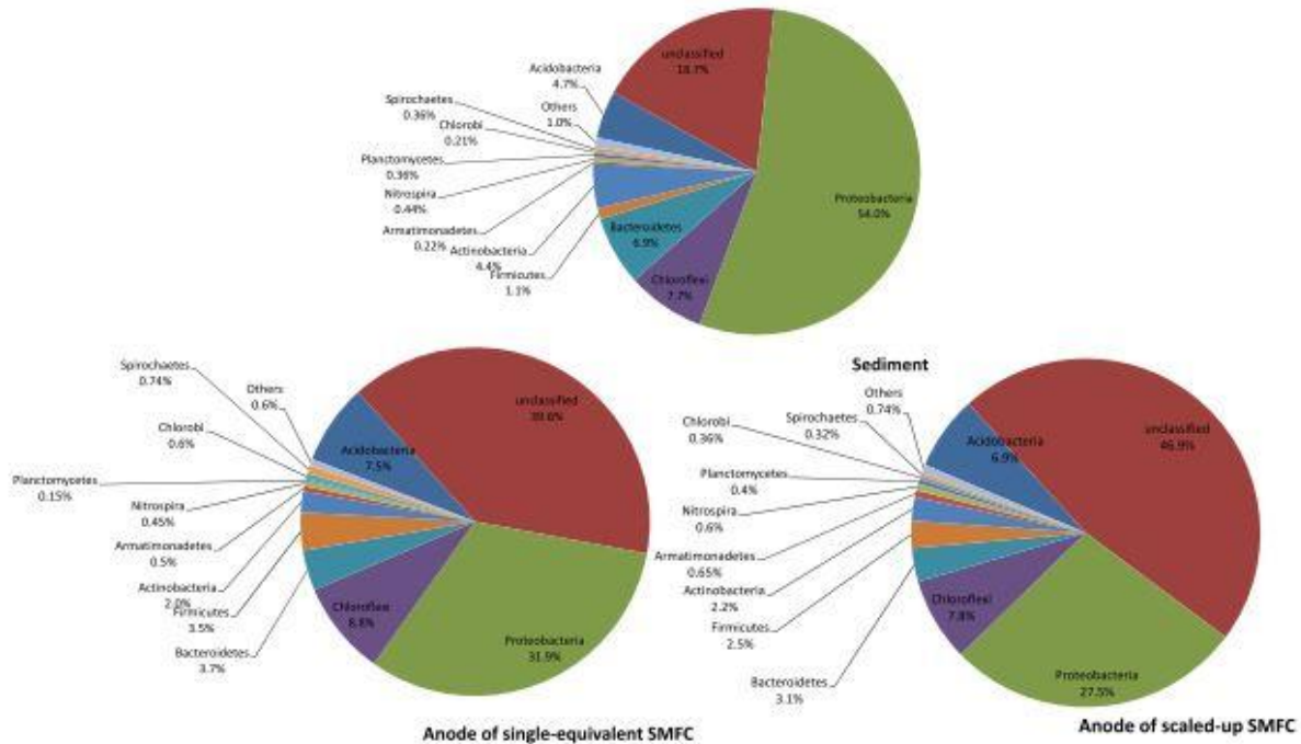
Figure 4. “Microbial community structure at the phyla level on anodes of the single-equivalent SMFC and the scaled-up SMFCs compared with the original sediment community.” 2
