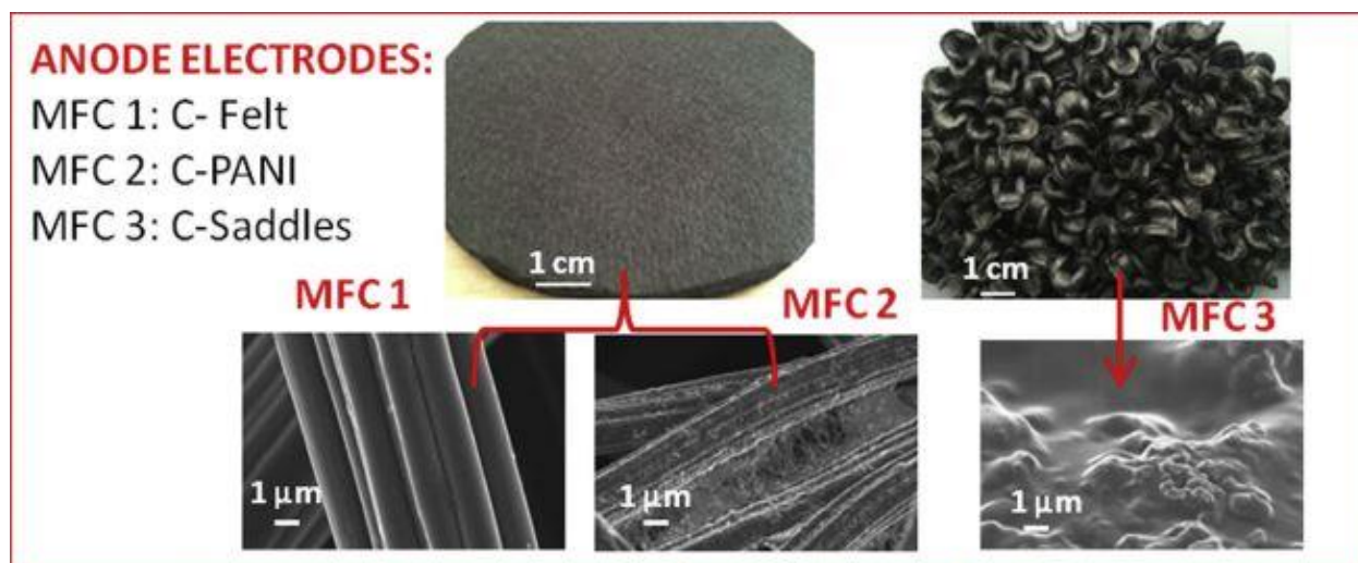
Figure 3. A macroscopic and microscopic view of carbon felt, carbon felt with polyaniline, and carbon-coated Berl saddles. Note the difference in appearance and texture. 7
