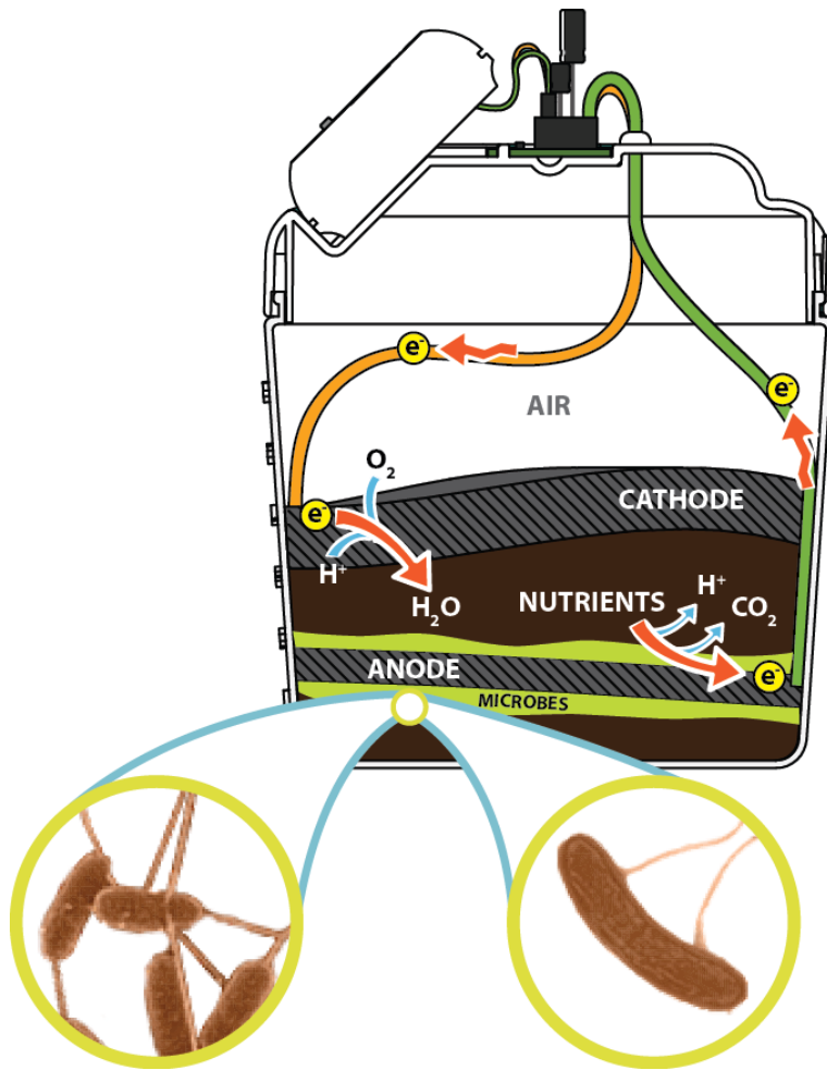
Figure 6. Schematic of a basic single-chamber air-cathode SMFC. Image from: http://www.fuelcellstore.com/mudwatt-microbial-fuel-cell-kit
