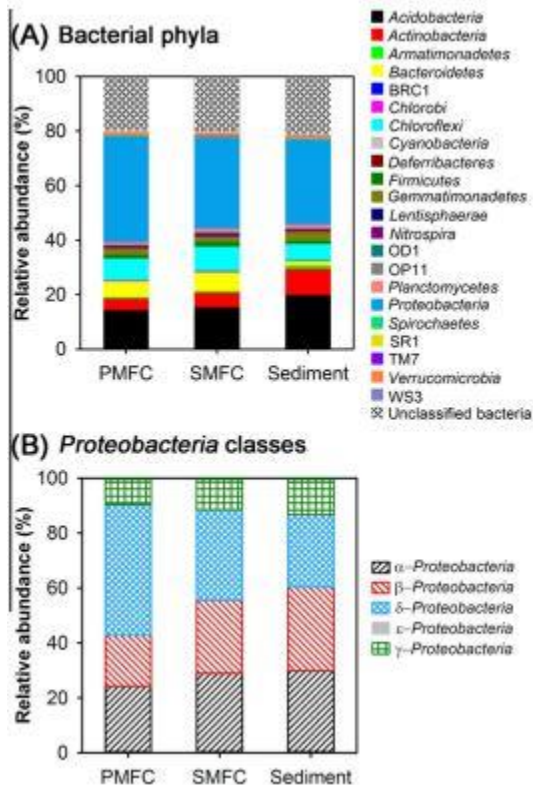
Figure 4. “Microbial community structure at the phyla level on anodes of the single-equivalent SMFC and the scaled-up SMFCs compared with the original sediment community.” 2
