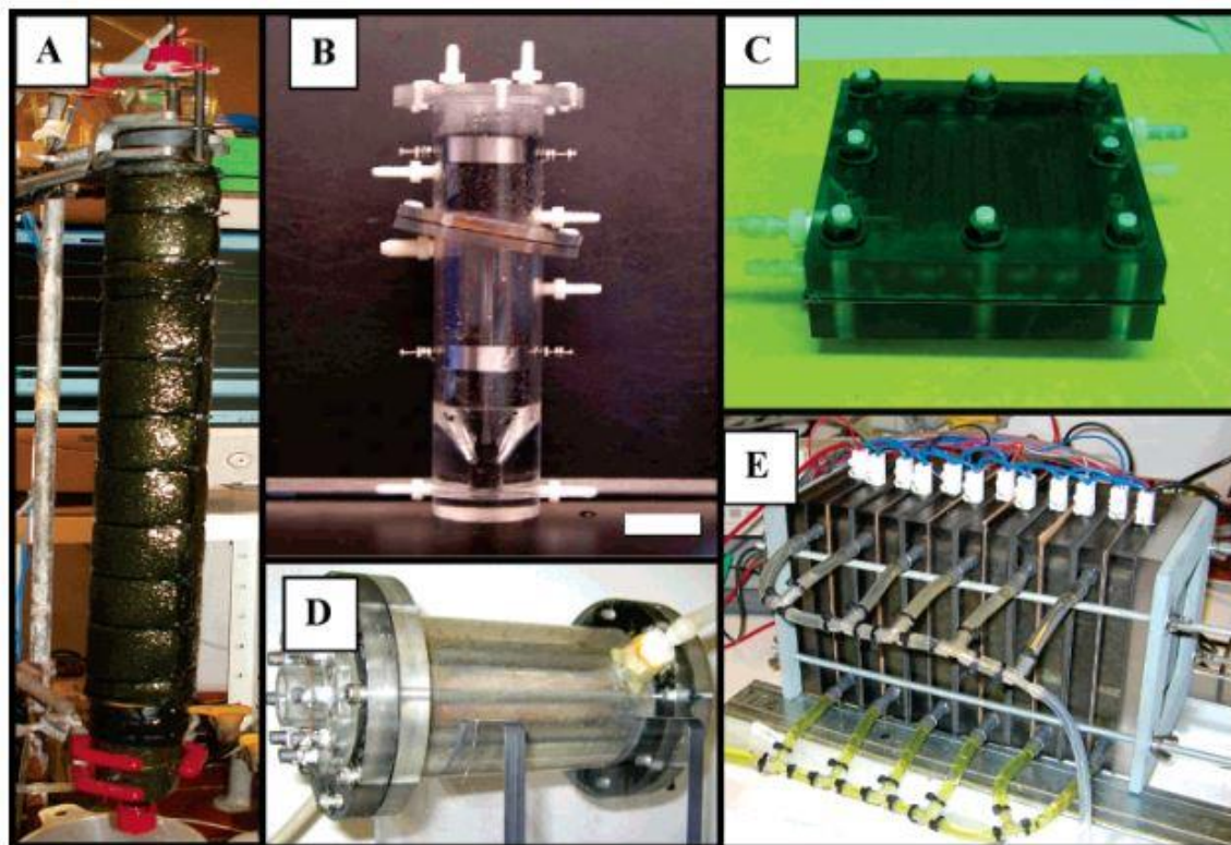
Figure 2. “MFCs used for continuous operation: (A) upflow, tubular type MFC with inner graphite bed anode and outer cathode; (B) upflow, tubular type MFC with anode below and cathode above, the membrane is inclined; (C) flat plate design where a channel is cut in the blocks so that liquid can flow in a serpentine pattern across the electrode; (D) single-chamber system with an inner concentric air cathode surrounded by a chamber containing graphite rods as anode; (E) stacked MFC, in which 6 separate MFCs are joined in one reactor block.” 1 [citations removed]
