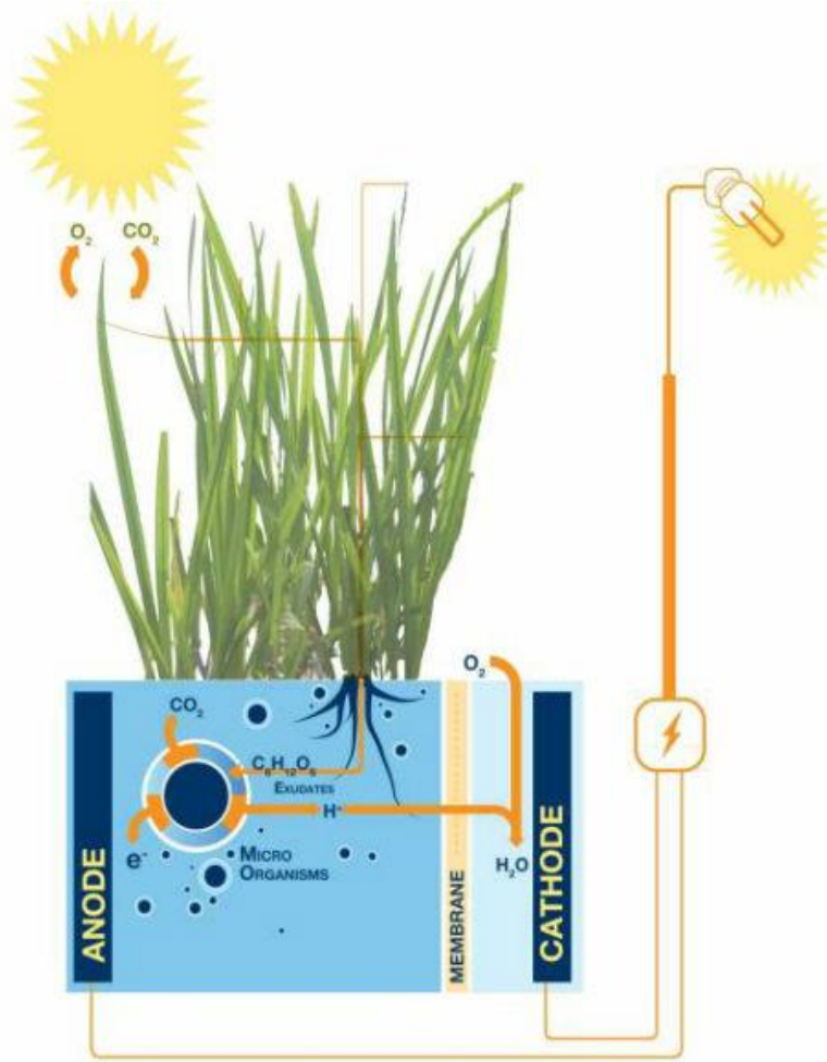
Figure 10. Schematic of the Plant-e PMFC. Image from: http://factor-tech.com/green-energy/1569-plant-power-the-new-technology-turning-green-roofs-into-living-power-plants/
