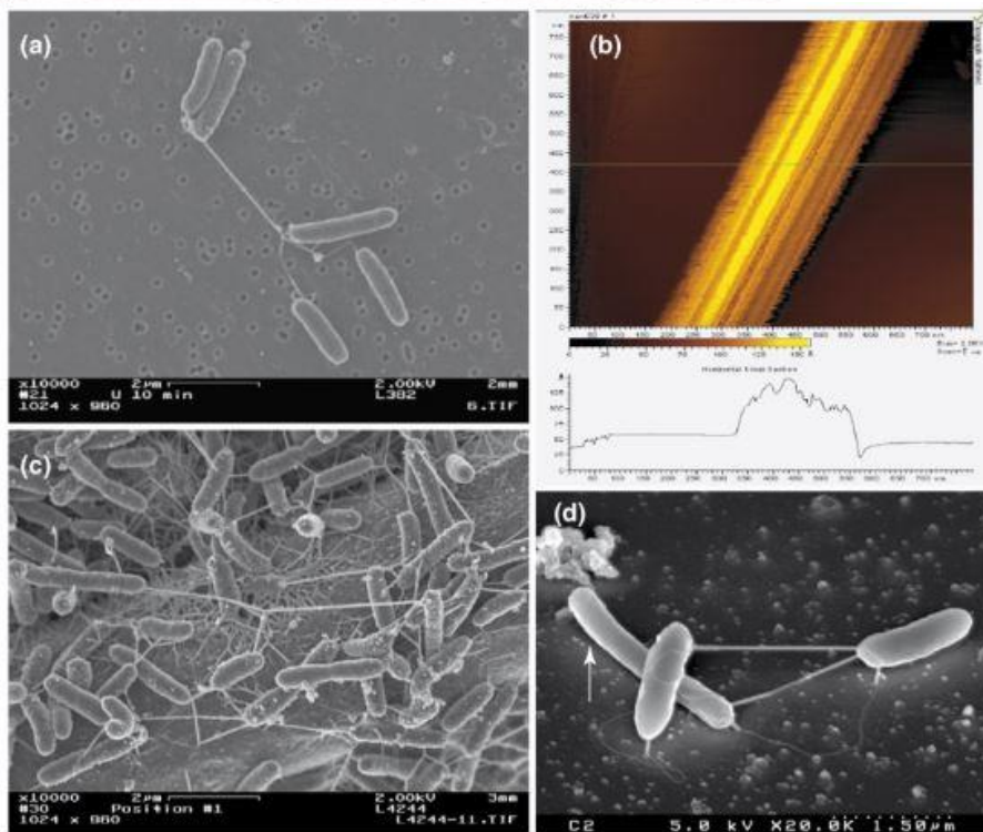
Figure 9. “(a) A scanning electron micrograph (SEM) of wild-type Shewanella oneidensis MR-1 grown under electron-acceptor-limited conditions, showing pilus-type nanowires that connect to other cells. (b) STM image of a single pilus-type nanowire from wild-type MR-1 (lateral diameter of 100 nm, topographic height of 5–10 nm) showing ridges and troughs running along the long axis of the structures consistent with a bundle of wires. The corresponding conductivity of the pilus as the tip moves over the indicated surface is shown beneath the STM image. (c) The anode from an MFC colonized by S. oneidensis MR-1. (d) An SEM image of Pelotomaculum thermopropionicum and Methanothermobacter thermautotrophicus (arrow) in methanogenic co-cultures showing pili connecting the two genera. Subsequent STM imaging has shown that the pili are conductive.” 12
