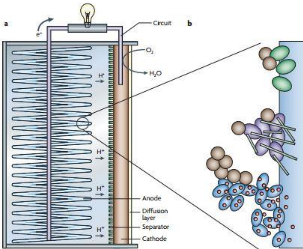
Figure 7. “Schematic of a microbial fuel cell (MFC) that contains an electrically conductive graphite fiber brush anode as the surface for bacterial growth and a flat carbon cloth cathode coated with a catalyst on the water-facing side. A diffusion layer, such as PTFE (polytetrafluoroethylene), is placed on the air-facing side to reduce water leakage, and a separator (or ion exchange membrane) is sometimes placed between the electrodes to allow charge transfer. O_2 is reduced to H_2O through a combination of electrons from the circuit and protons in the water. b| shows the different types of microorganisms in an anodic biofilm, including exoelectrogens that transfer electrons by direct contact (green), produce nanowires (purple) and use endogenous (and therefore self-produced) mediators (blue). other non-exoelectrogenic bacteria (brown) that live off the products produced by other bacteria or possibly use mediators or nanowires produced by other microorganisms can also be present.” 11
