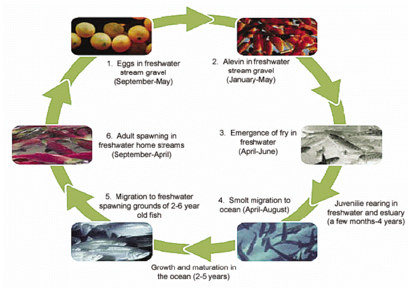
Diagram 2 – Illustration of the Anadromous Life-Cycle of Salmon
