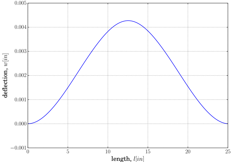
Figure 4.19: Deflection along length for a clamped-clamped beam at t = 0.65sec
