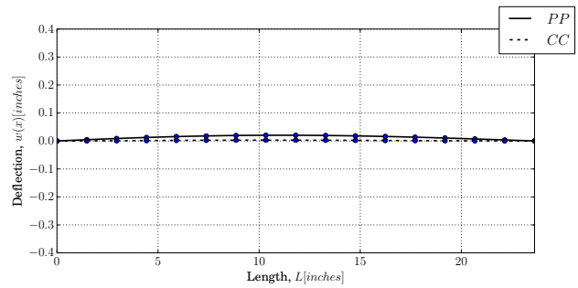
(b) Deflection
