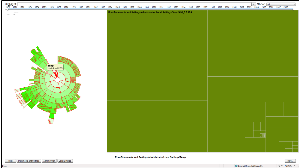
Figure 21: Temp is clicked, child nodes of Temp visualized in treemap Visualization.
