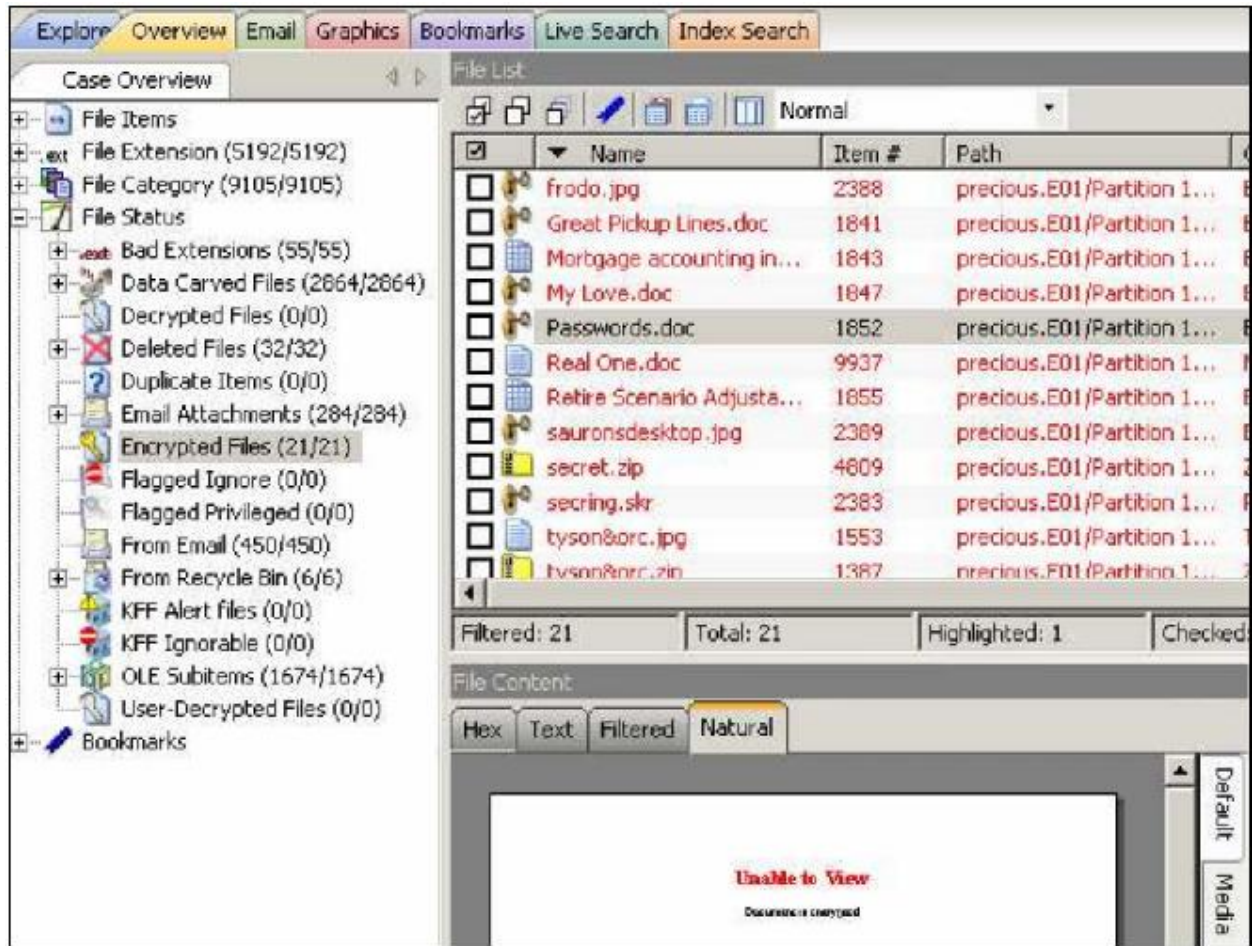
Figure 2: FTK interface.
