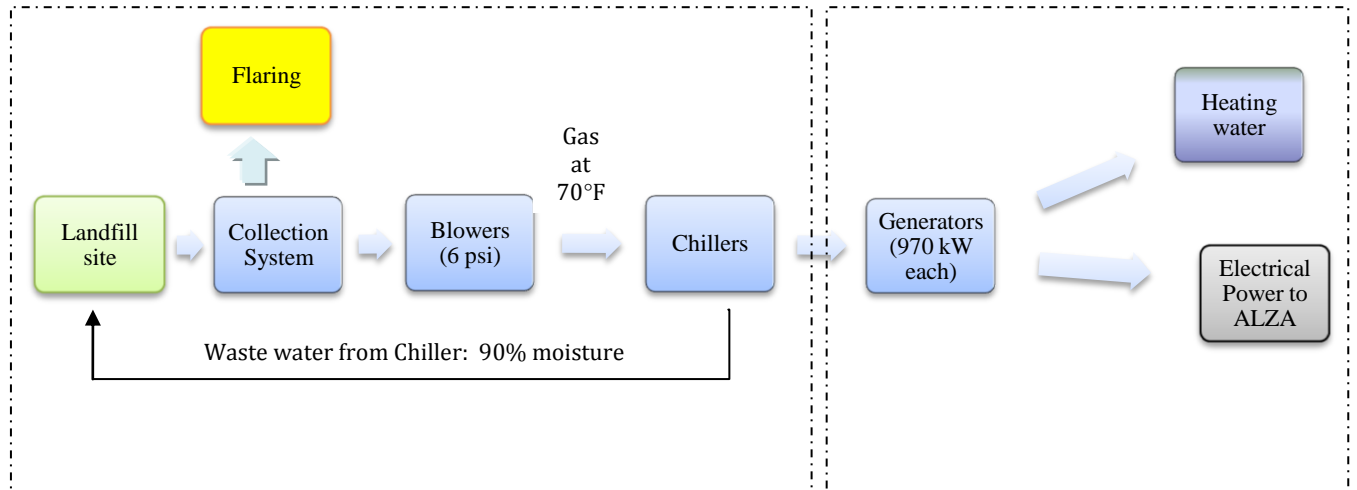
Figure 6.1: The process of Landfill gas being collected for both Electrical and Heating utilization at ALZA Pharmaceuticals, San Francisco
