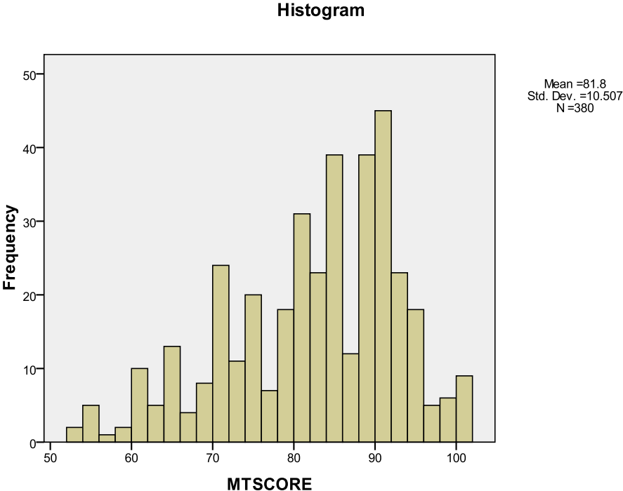
Figure 4.1 Normality Test
