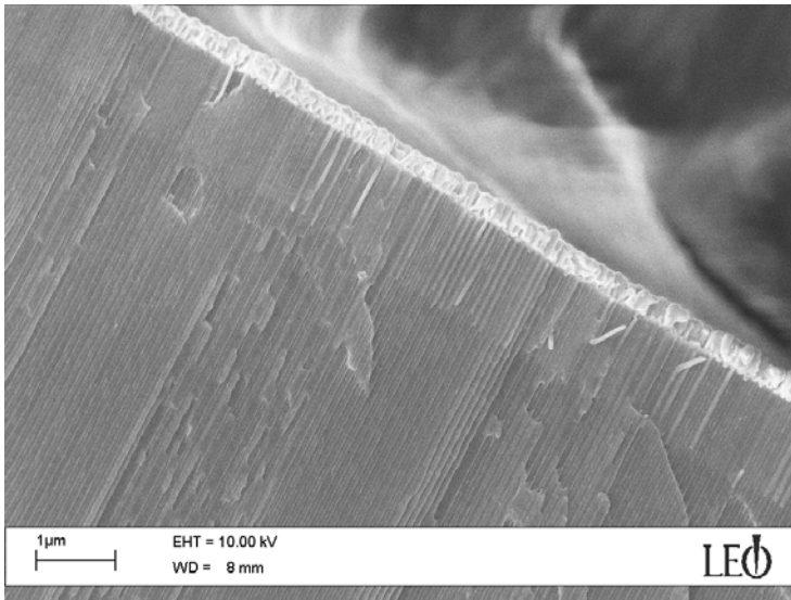
Figure 2.4 SEM image of Ni nanowire arrays of 60 nm diameter and 100 nm interpore distance.
