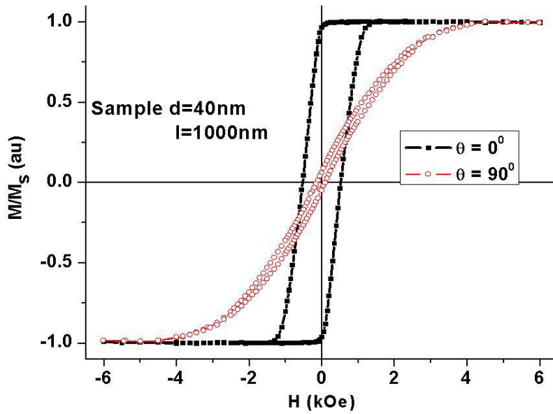
Figure 3.5 The hysteresis curve for the sample d40l1000 at 0^0 and 90^0
