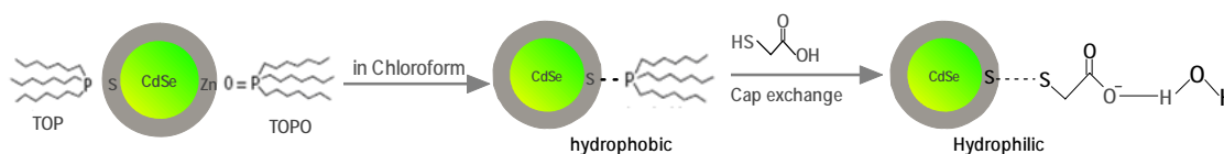
Figure 3.7 Schematic of synthesis of QD-mercaptopropionic acids
