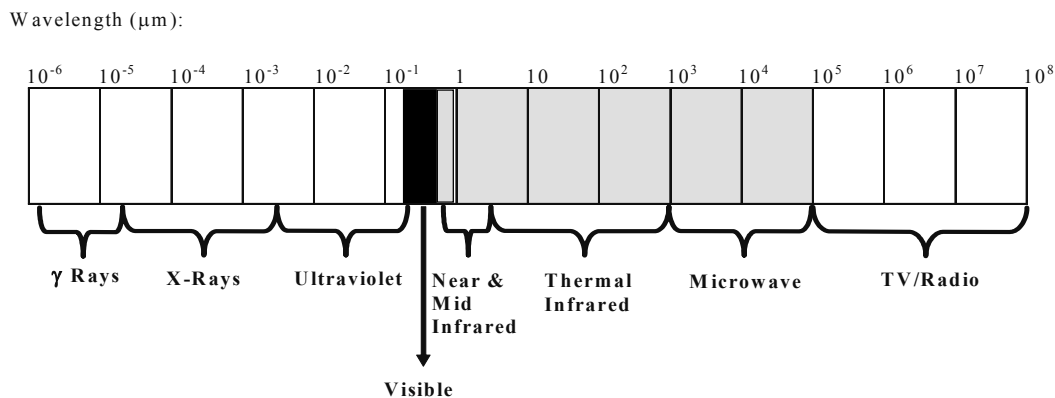
Fig.14: The electromagnetic spectrum (modified from Sears and Zemansky, 1973)
