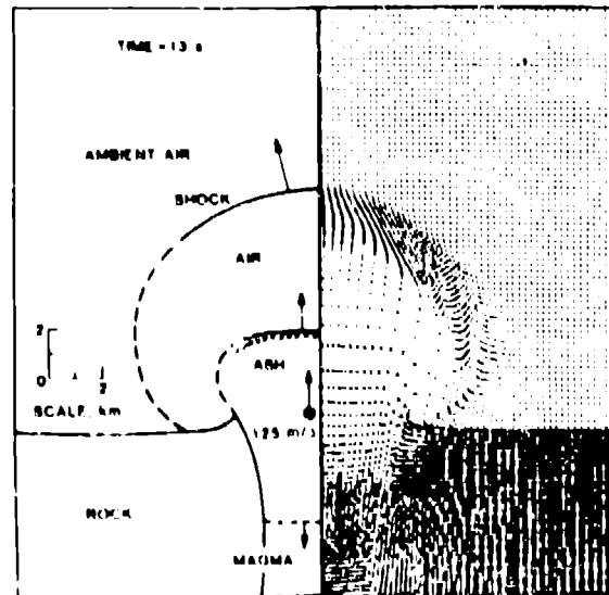
Figure 3. Representation of a volcanic blast eruption predicted by numerical simulation of an overpressured eruption. The right hand side of the plot shows calculated ash and atmospheric marker particles (Wohletz and others, 1984).
