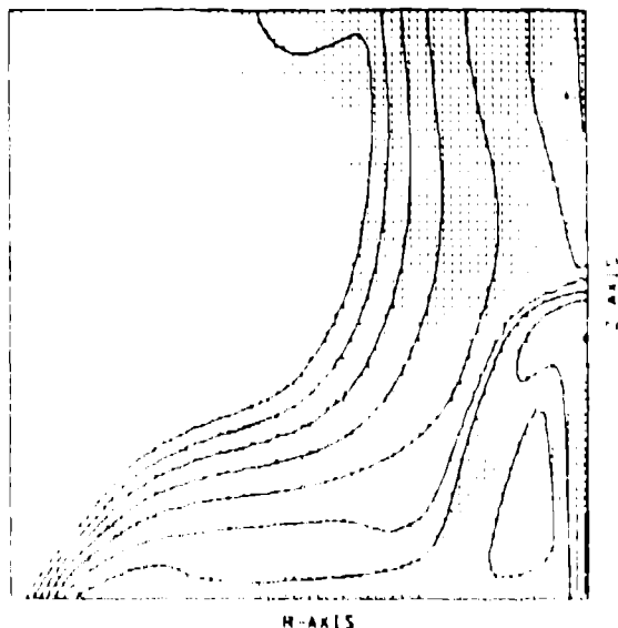
Figure 5. A simulated pyroclastic flow is shown as in Fig. 4 with contours of ash concentration. For each point in the grid, various flow parameters may be obtained for hazard assessment.
