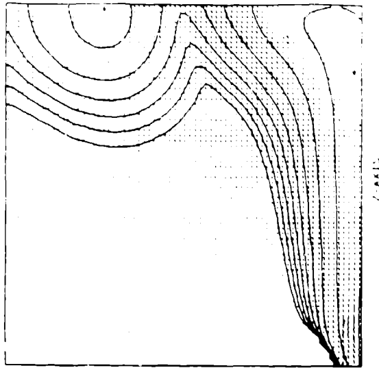
Figure 4. Simulated Plinian eruption column portrayed as contours of volume fraction of volcanic ash. Dots and lines are nodal dust velocity vectors. Note axisymmetry around the vent (lower right) and the 7X7 km calculational regime.
