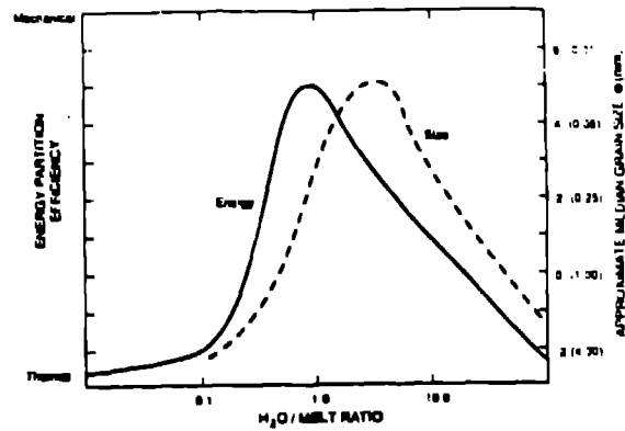
Figure 1. Results of water/magma interaction experiments showing the affect of water:melt mass ratio on explosive energy and fragment size (adapted from Frazzetta et al., 1983).
