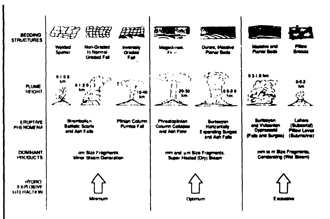
Figure 2 Relationship of volcanic activity to the abundance of ground water in and around the volcano (adapted from Sheridan and Wohletz, 1983)
