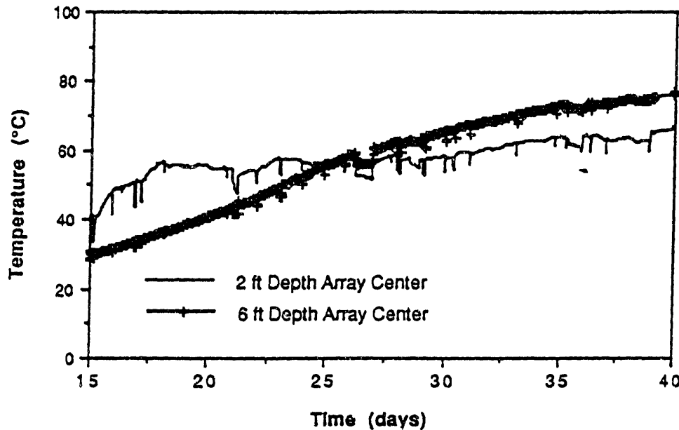
Figure 3 - Temperatures at 2 ft and 6 ft Depth in Center of Array
