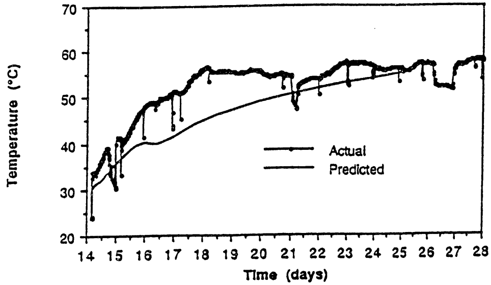
Figure 4 - Predicted vs Actual Temperature at 2 ft Depth
