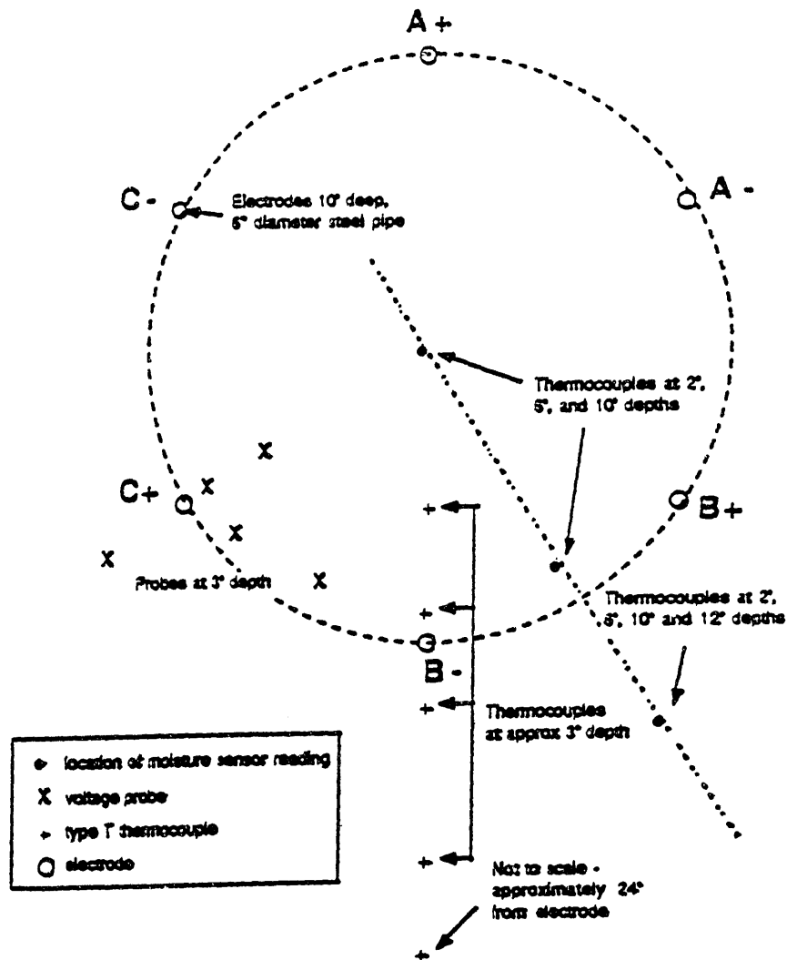
Figure 1 - Six-Phase Heating Field Test Layout
