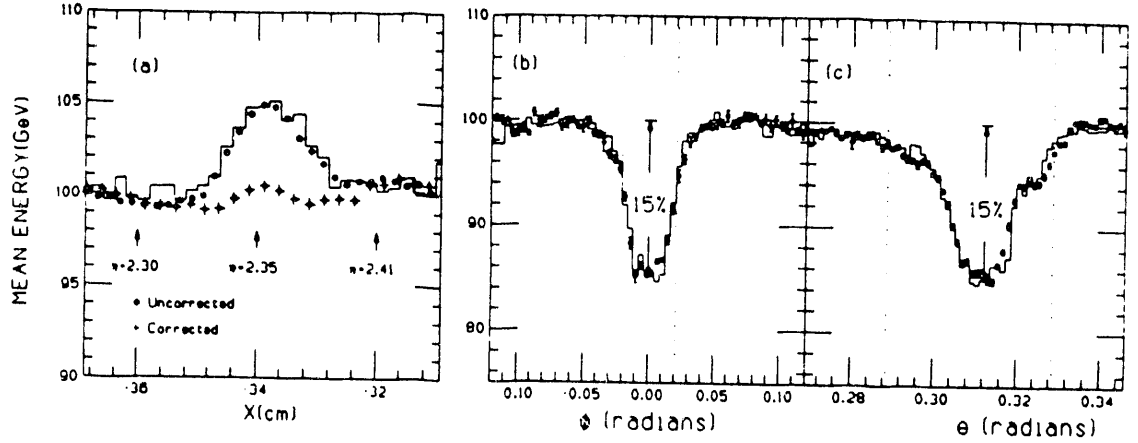
Figure 5: Calorimeter response to 100 GeV e^- s. (a) Mean energy vs x before and after the correction in the vicinity of the uranium gap. (b) Mean energy vs \phi and (c) Mean energy vs \theta in the vicinity of the tie-rod. The points are the data and the histograms are from the Monte Carlo simulation.
