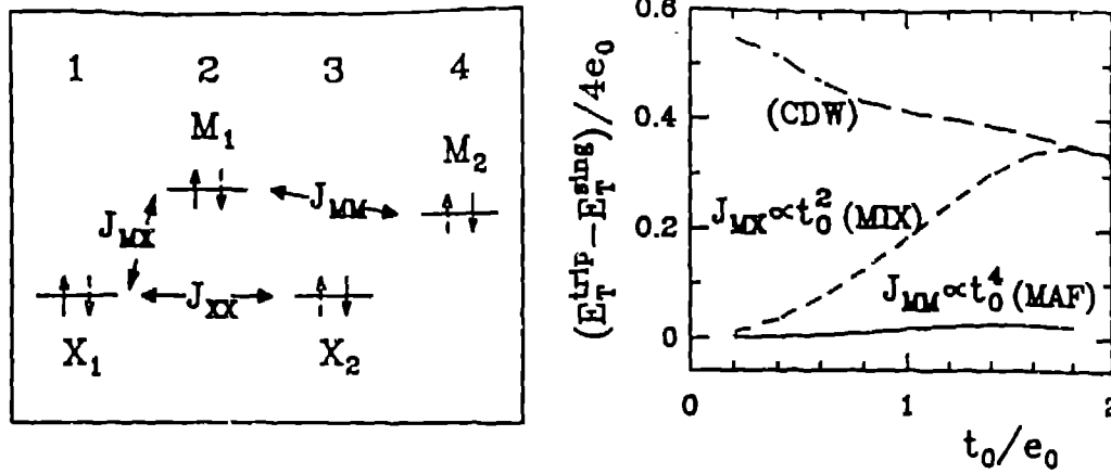
Fig. 2 (left). Schematic energy level diagram in the strongly correlated limit showing frustration of the effective antiferromagnetic couplings caused by MX hybridization.
