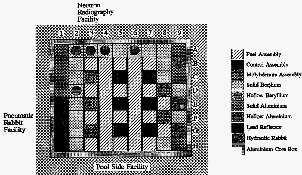
Figure 3: SAFARI-1 Core
