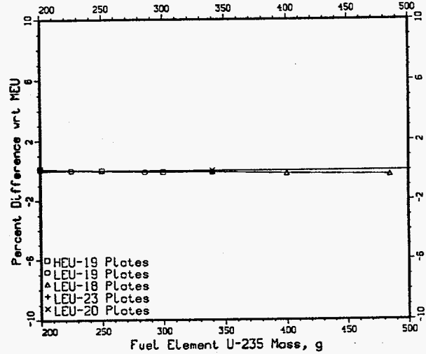
Figure 6. THERMAL-TO-TOTAL FLUX RATIO: POOL SIDE
