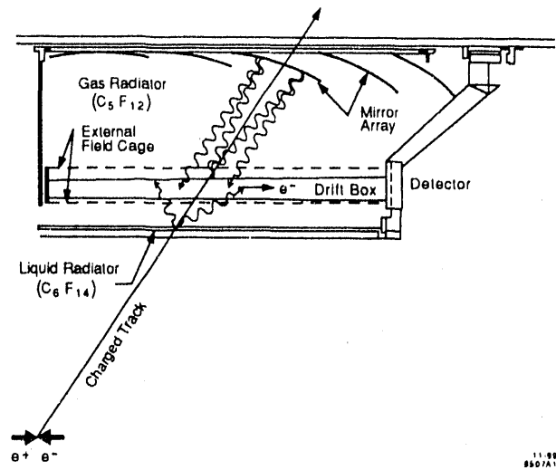
Fig. 1 Principal Components of the SLD Barrel CRID.
