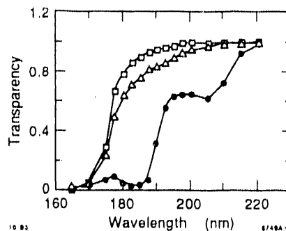
Fig. 12 Transmission of 1 cm of cleaned liquid from (squares), freon exposed to DP-190 for 107 days (circles), and freon exposed to G-10 for 128 days (triangles).
