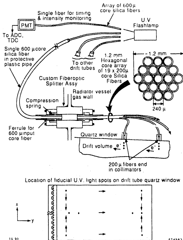
Fig. 3. The fiber optic calibration system.
