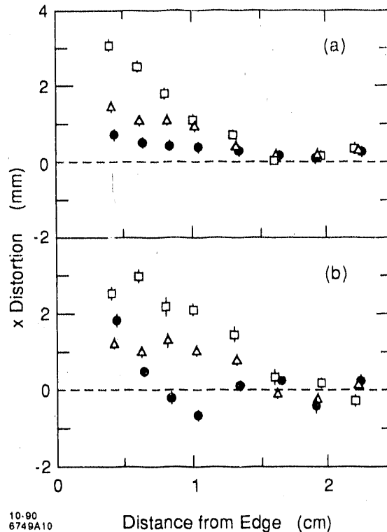
Fig. 10 x -distortion measurements as a function of expected x -position near the top (squares), middle (triangles) and bottom (solid circles) of a drift box, and for (a) 60 and (b) 117 cm drift.
