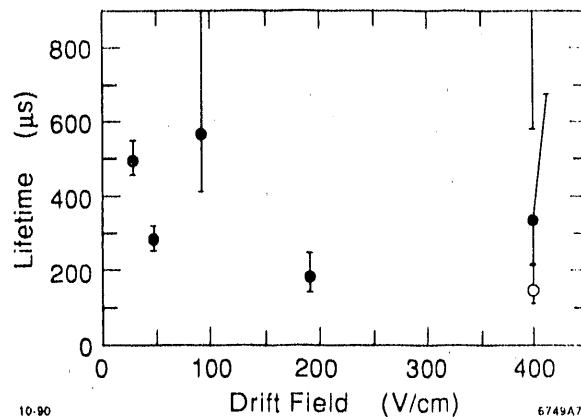
Fig. 11 Electron lifetime measured for various drift fields. The open circle is a measurement for pure ethane, the rest for ethane plus 0.1% TMAE.
