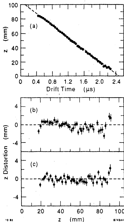
Fig. 5 A z -distortion measurement from the central optical fiber: (a) average depth versus arrival time; (b) residuals versus expected depth; (c) as (b), but ungated.
