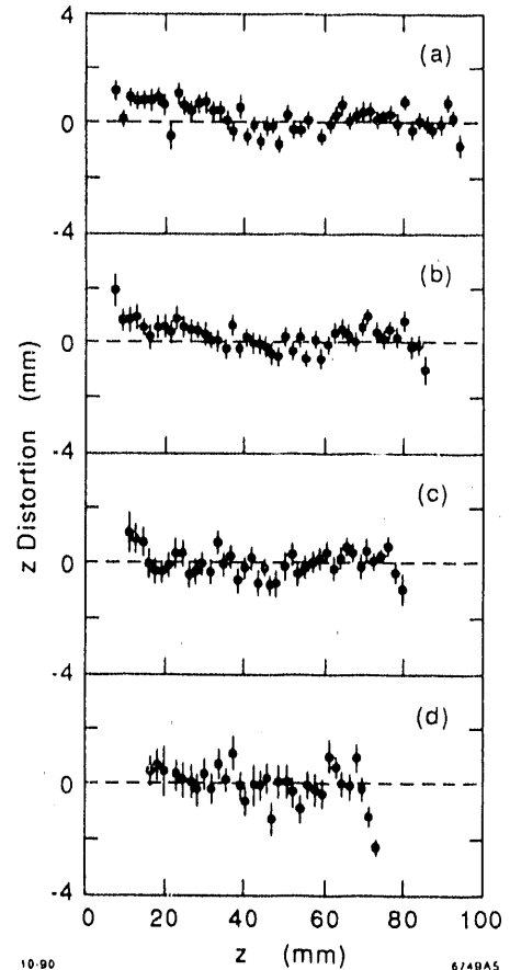
Fig. 8 z -distortion measurements along the box centerline for drift distances of (a) 7, (b) 42, (c) 78, and (d) 117 cm.
