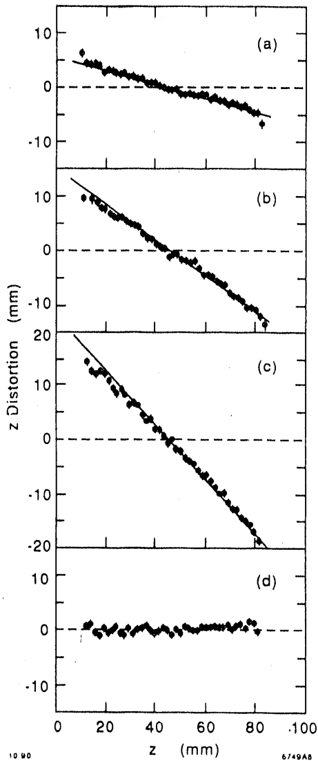
Fig. 7 z -distortion measured with space-charge densities of (a) 0.5 , (b) 1.5 , (c) 2.5 \times 10^6 ions per \text{cm}^3 (the solid lines are results of an electrostatic simulation), and (d) measured under the same conditions as (c) except that the gating has been turned on.
