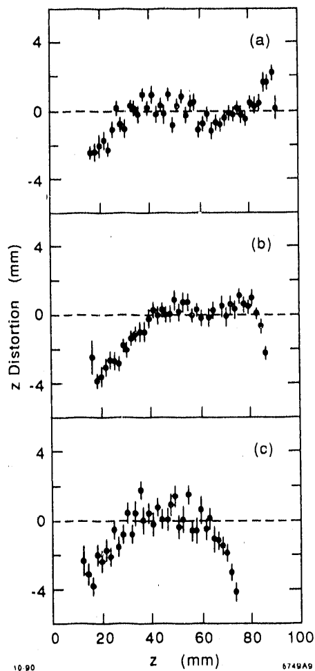
Fig. 9 z -distortion measurements 1.5 cm from one side of a drift box for drift distances of (a) 42, (b) 78, and (c) 117 cm.
