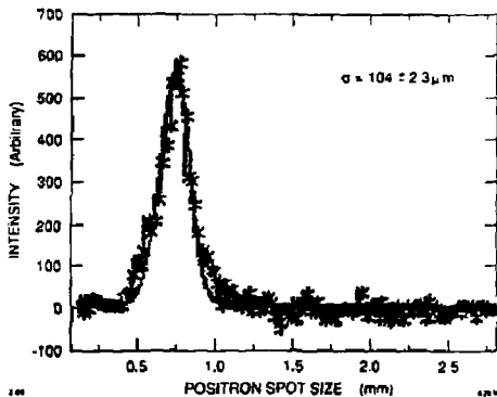
Fig. 8. Projection of a digitized positron beam profile with width \sigma_x = 104 \pm 2.3 \mu\text{m} (statistical error only).
