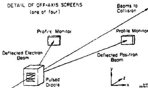
Fig. 7. Detail of one of four sets of off-axis profile monitors used in the transverse beam profile monitoring system.
