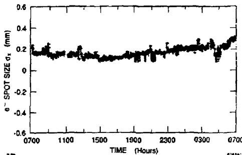
Fig. 9. Measurements of the electron spot size (width \sigma_x of projection) taken at four-minute intervals over a 24-hour period.
