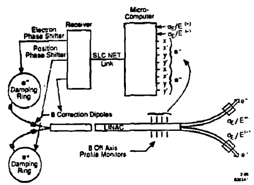
Fig. 1. Overview of the transverse beam profile and energy spread monitoring and feedback systems.
