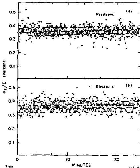
Fig. 5. Energy spread of the linac as a function of time without feedback. Measurements are made at 0.5 Hz.
