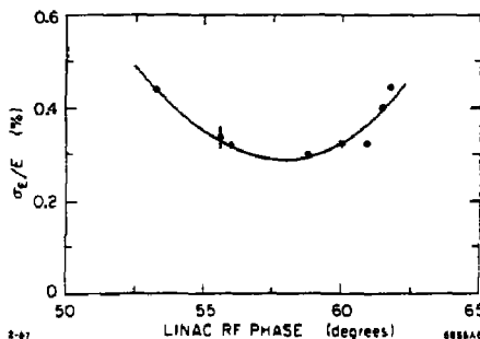
Fig. 6. Measurement of the bunch energy spread, \sigma_E/E , as a function of the RF phase of the Linac.
