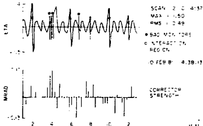
Fig. 3. Typical vertical dispersion function before correction.
