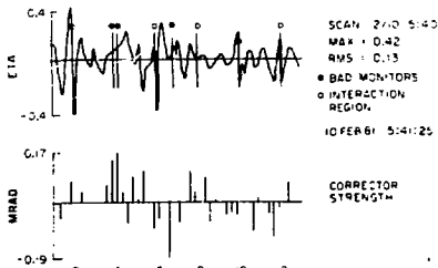
Fig. 4. Vertical dispersion function after correction.
