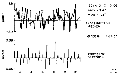
Fig. 2. Vertical orbit after global correction using method 2.
