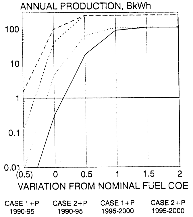
FIGURE 7. THE SENSITIVITY OF WIND PENETRATION TO VARIATIONS IN FUEL COSTS
