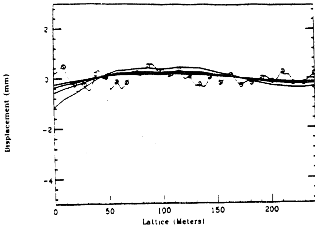
Figure 2. Optimization of injection parameters.
