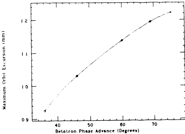
Figure 5. Betatron phase advance effects on orbit deviations.
