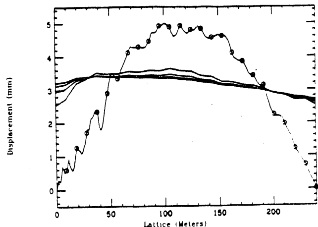
Figure 3. Systematic error with two fiducials.
