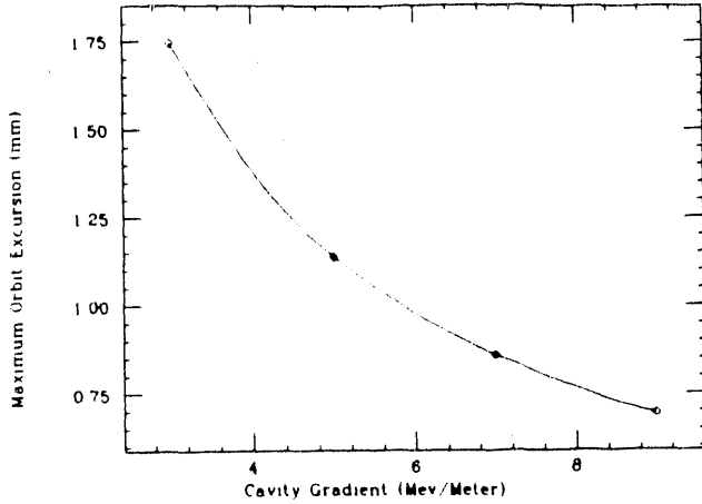
Figure 4. Cavity gradient effects on orbit deviations.
