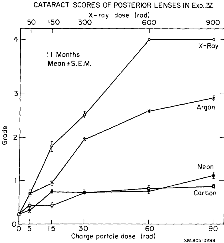
Figure 6. Average severity of posterior lens cataracts induced in mice eleven months after irradiation with plateau argon, neon or carbon ions. The bars indicate the standard errors of the mean. The average score among controls was nil.
