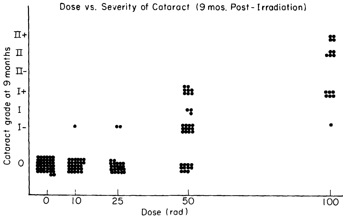
Figure 2. Severity of cataracts at nine months in LAF mice irradiated with spread Bragg peak argon ions (Experiment II). Each dot indicates one animal.
