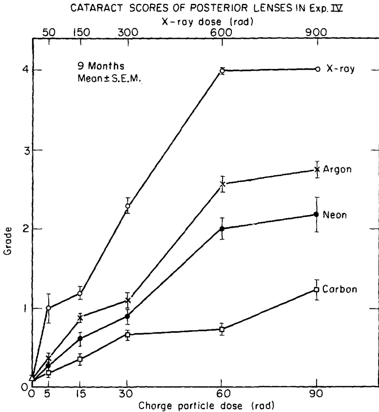
Figure 5 Average severity of posterior lens cataracts in mice nine months after irradiation with plateau argon, neon or carbon ions. The bars indicate the standard errors of the mean. The average score among controls was nil.
