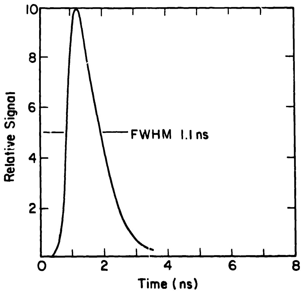
Fig. 2. Current vs. time for the Febotron 706 electron beam after filtration by 103 \text{ mg/cm}^2 aluminum.
