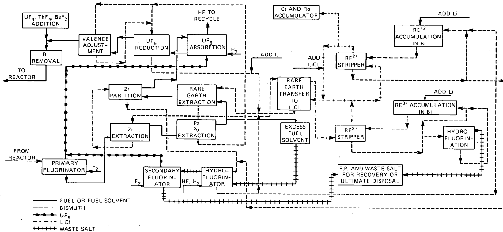
Fig. 6.4. Preliminary flowsheet for fuel processing in a DMSR.
