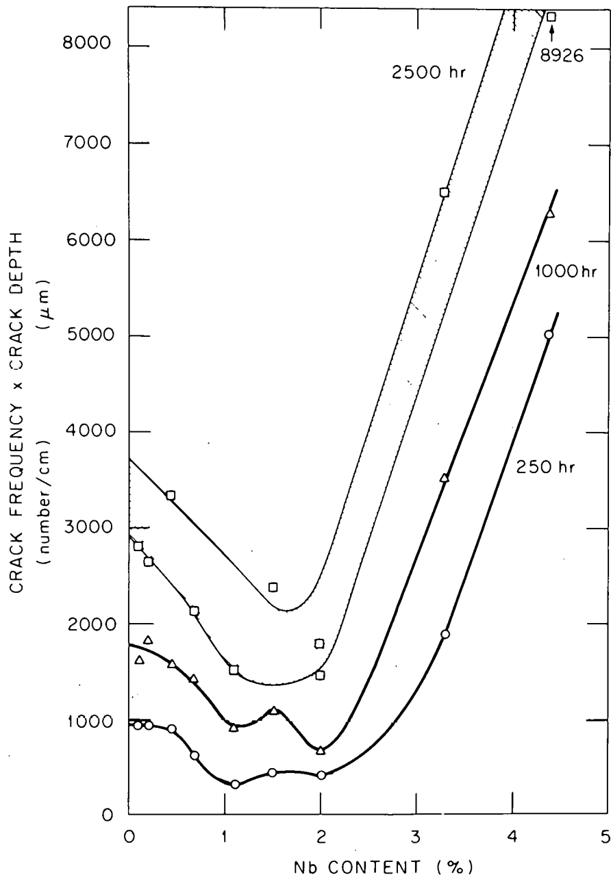
Fig. 7.1. Variations of severity of cracking with niobium content. Samples were exposed for indicated times to salt containing \text{Cr}_3\text{Te}_4 and \text{Cr}_5\text{Te}_6 at 700^\circ\text{C} .
