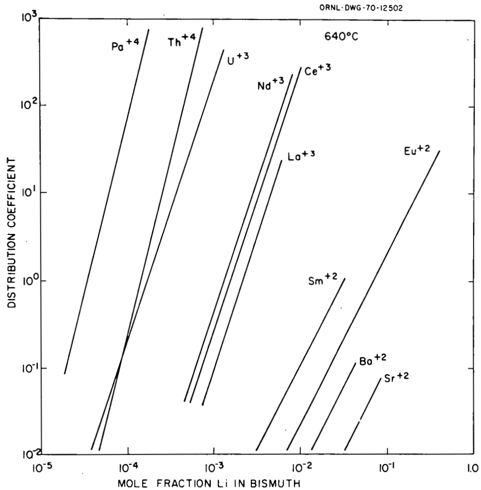
Fig. 6.2. Distribution data between lithium chloride and bismuth.
