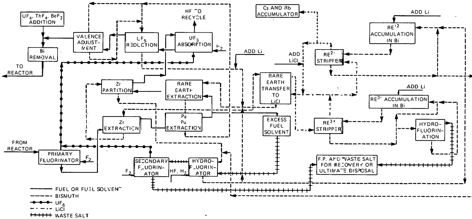
Fig. S.1. Proposed DMSR fuel processing flowsheet.
