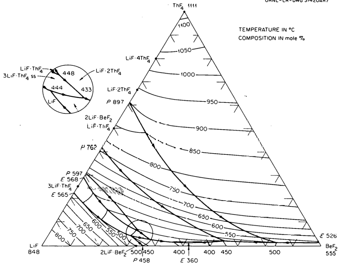
Fig. 3.1. The system LiF-BeF 2 -ThF 4 .
