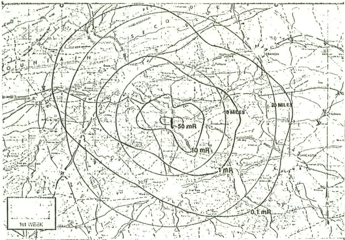
FIGURE 3: Estimated External Exposure for the First week Following the Accident from TLD Data
