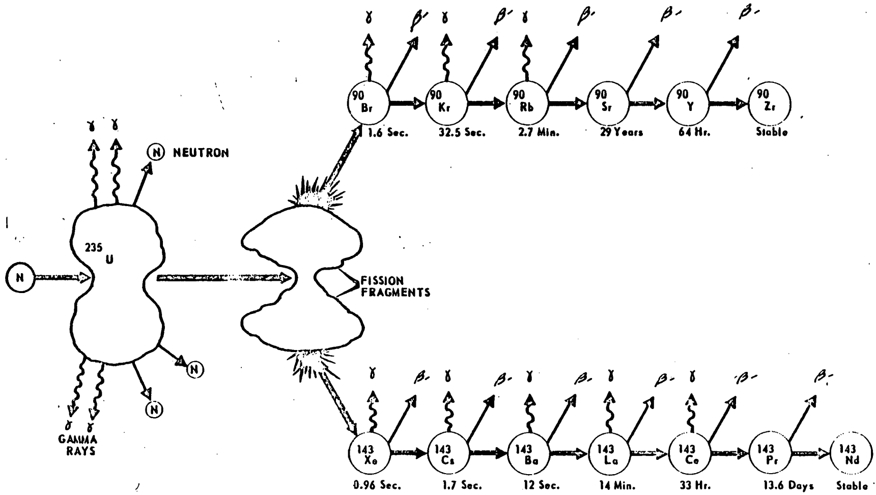
URANIUM FISSION AND BETA DECAY CHAINS
