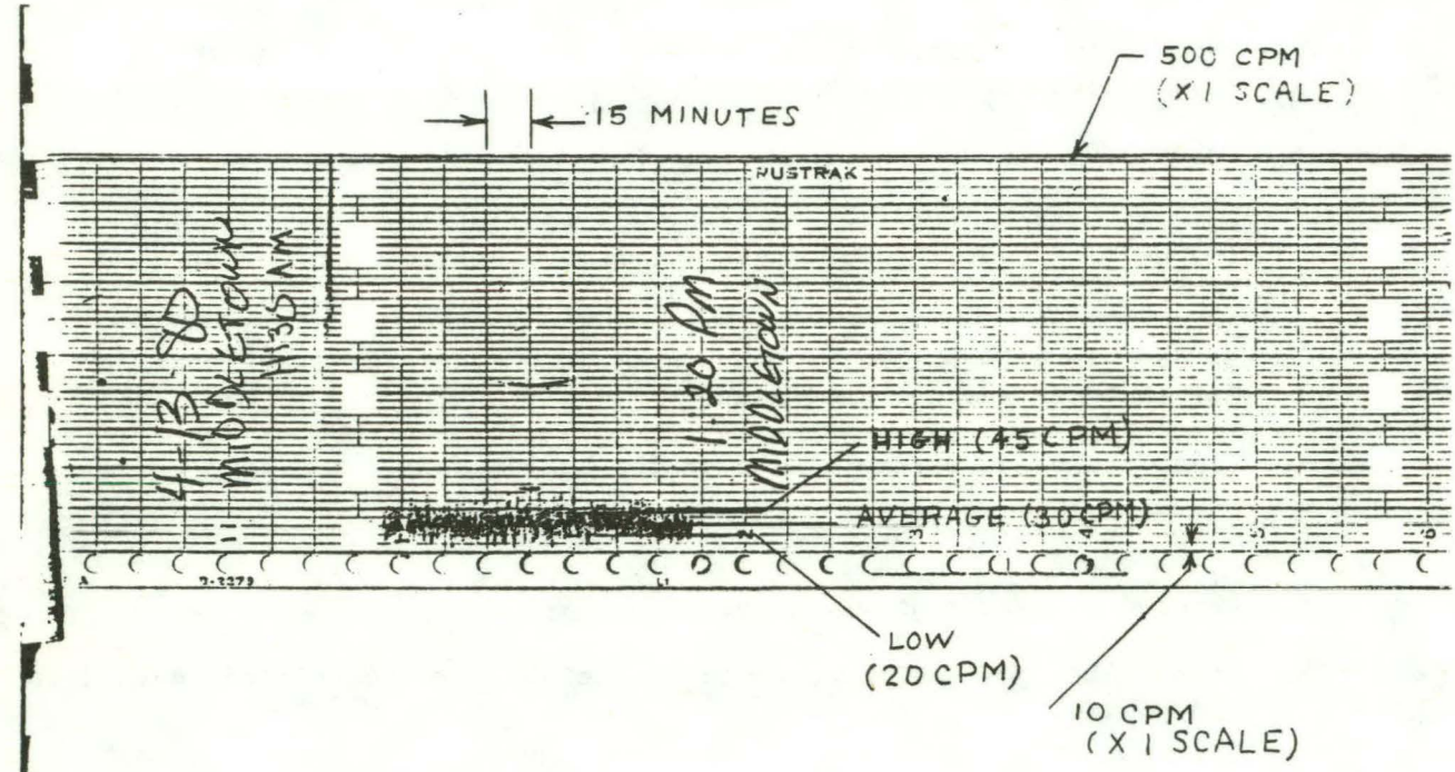
FIG 1. LUDLUM CHART OUTPUT (BACKGROUND)
